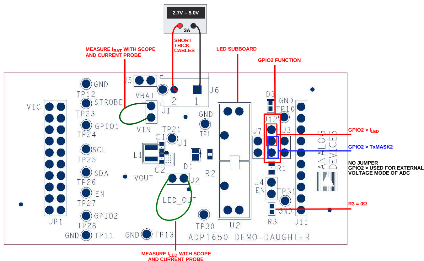
Figure 10. Demonstration Daughterboard
