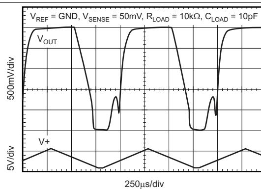
Figure 20. Start-Up Transient Response
