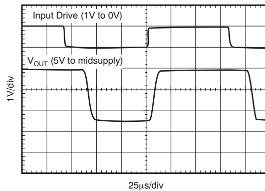
Figure 31. Input Overload
