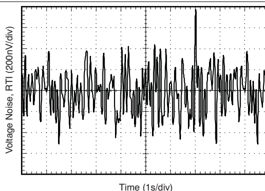
Figure 14. INA282 0.1-Hz to 10-Hz Voltage Noise, RTI
