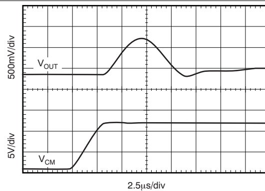
Figure 22. 12-V Common-Mode Step Response
