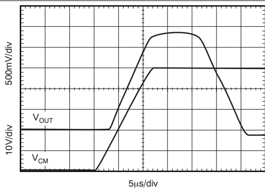
Figure 25. 50-V Common-Mode Step Response
