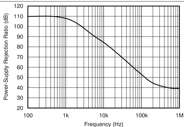
Figure 2. INA282 PSRR (RTI) vs Frequency
