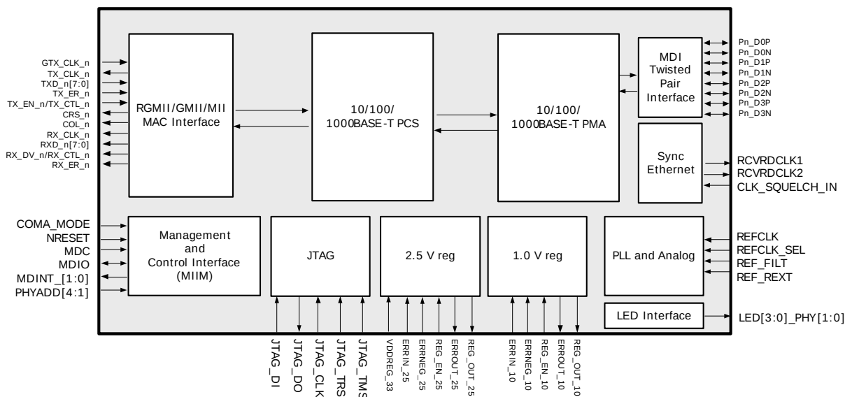
Figure 2 • Block Diagram
