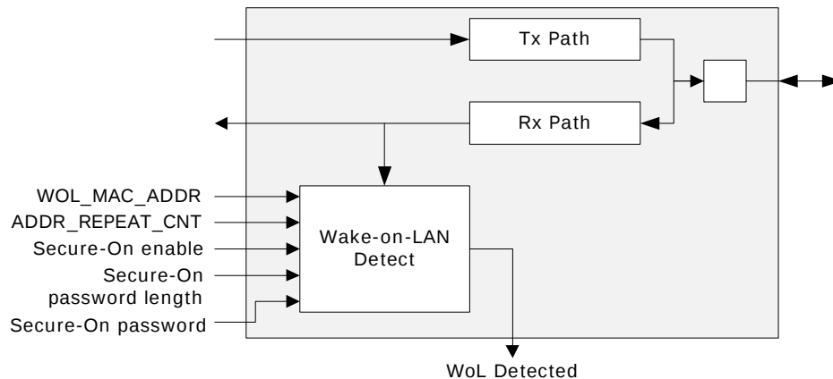
Figure 3 • Wake-on-LAN Functionality
