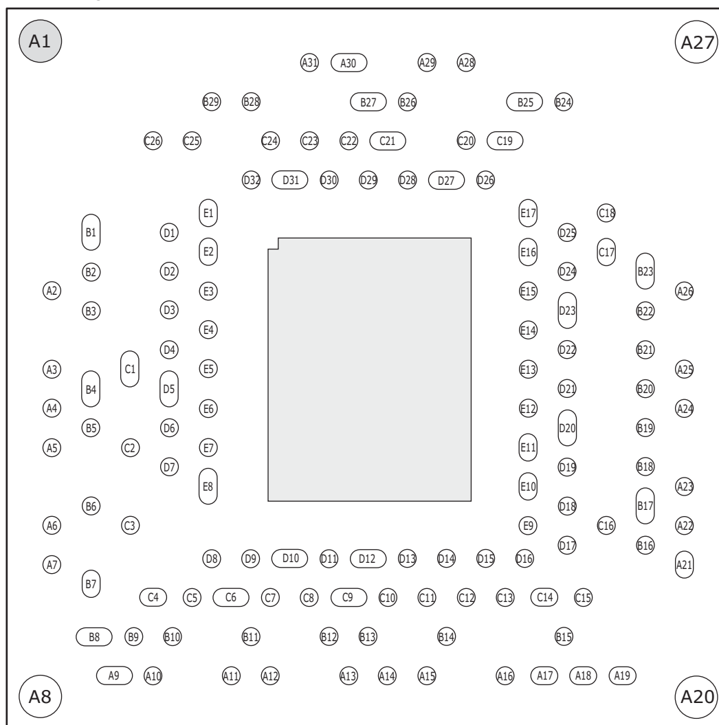
Figure 26 • Pin Diagram
