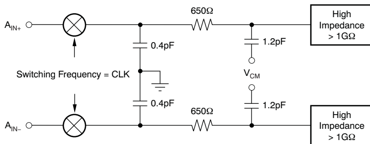
Figure 28. Input Impedance of the ADS1204
