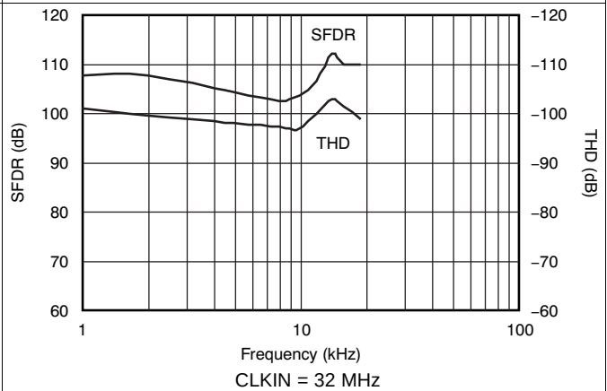
Figure 17. SFDR and THD vs Input Frequency
