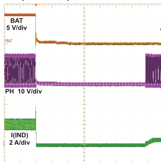
Figure 12. Short Battery
