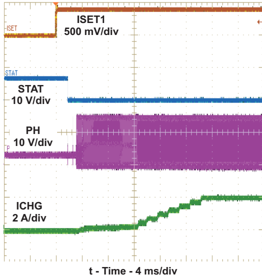
Figure 7. Charge Enable
