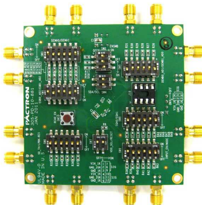
Figure 2. DS100KR401EVK (Bottom View)
