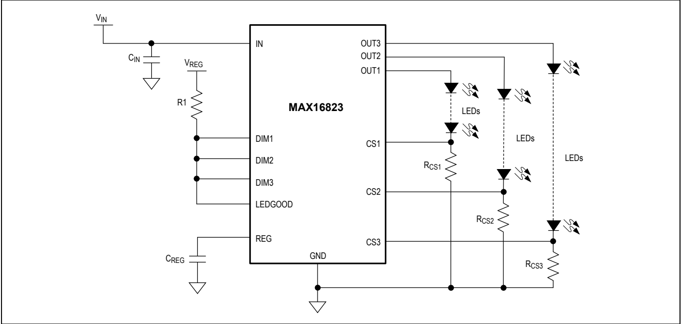
Figure 3. Output_Latch-Off
