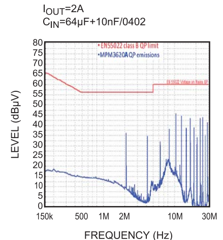
Conduction-EMI
