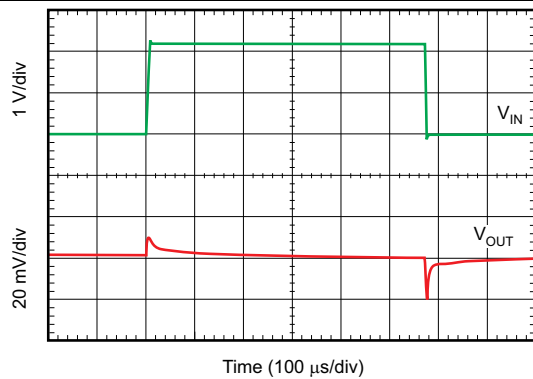
Figure 37. Line Transient Response
