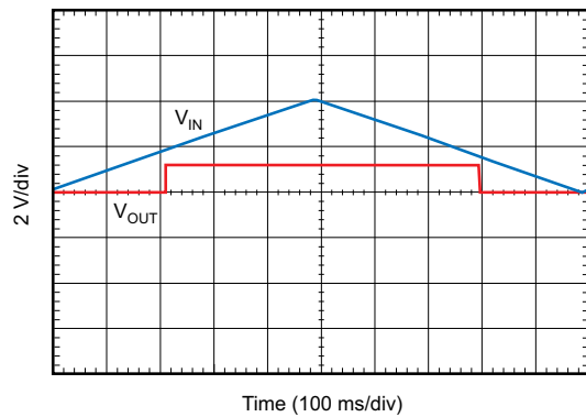
Figure 39. Line Transient Response
