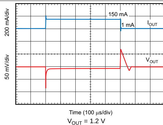
Figure 30. Load Transient Response
