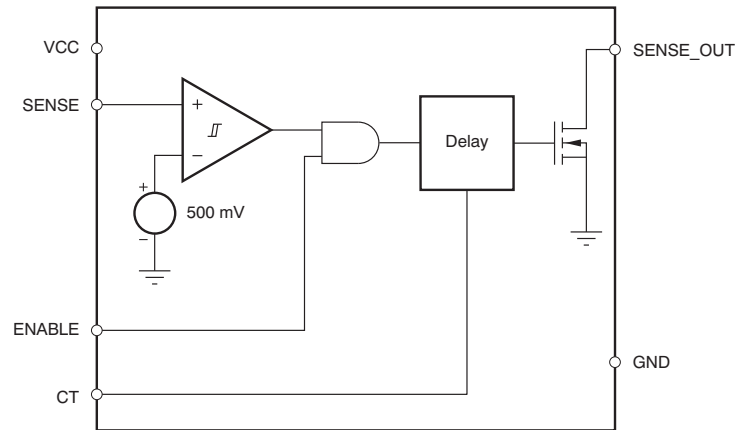
Figure 19. TPS3897A Block Diagram
