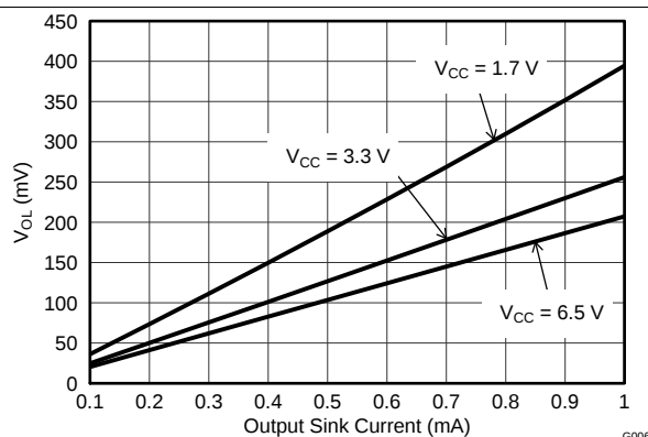
Figure 10. Output Voltage Low vs Output Current (0 mA to 1 mA)
