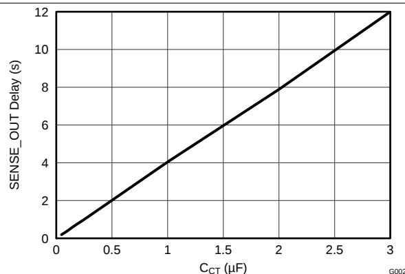
Figure 6. SENSE_OUT Time-Out Period vs C_{CT}
