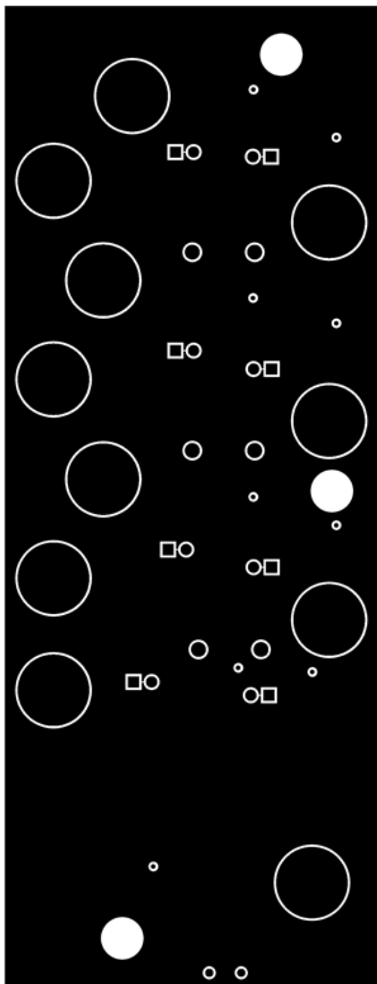
Figure 6. Layer 2 Copper
