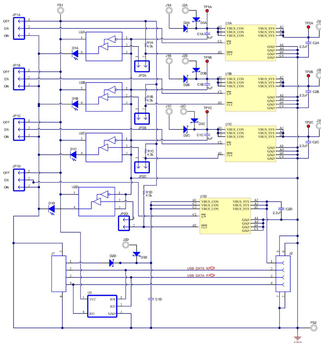
Figure 3. TPD1S414EVM Schematic
