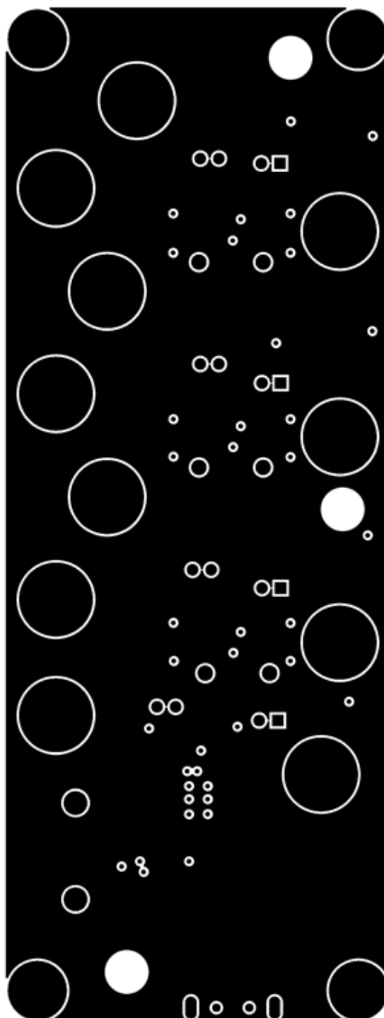
Figure 7. Layer 3 Copper
