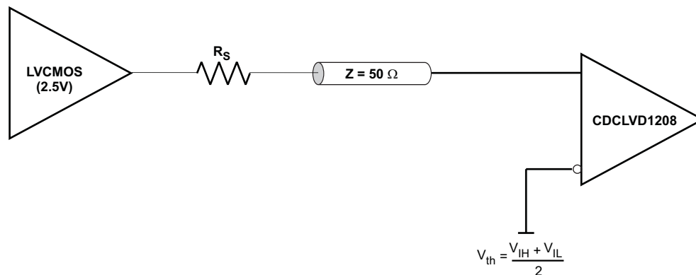
Figure 15. 2.5-V LVCMOS Clock Driver Connected to CDCLVD1208 Input
