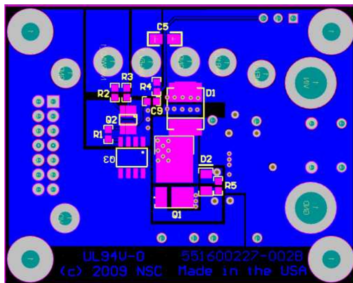
Figure 3. Bottom Layer
