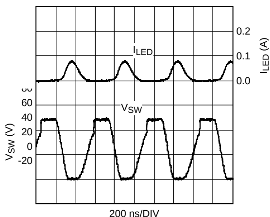
Figure 10. Analog dimming minimum ( V_{ADJ} = 0V )
