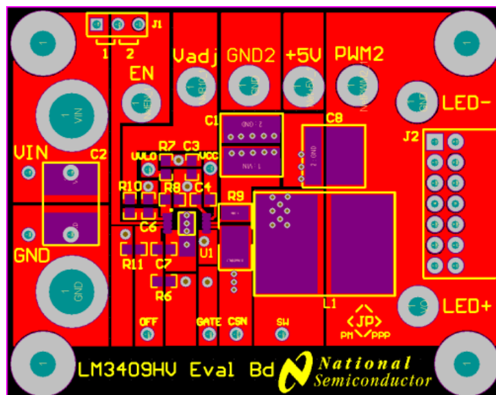
Figure 2. Top Layer
