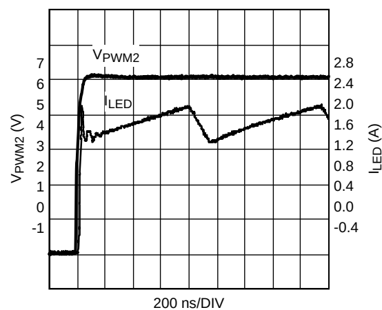
Figure 9. 100kHz 50% External FET PWM dimming (rising edge)
