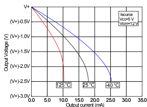
Figure 12. Positive output voltage swing vs output current V_{CC} = 5 V
