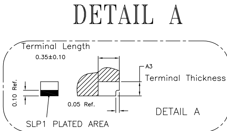
Figure 31. QFN10 detail A package outline
