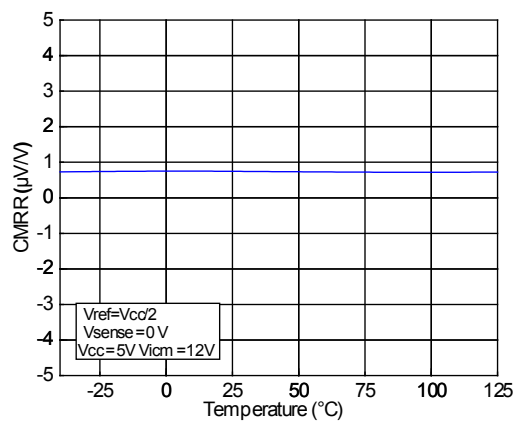
Figure 6. Common mode rejection ratio vs temperature
