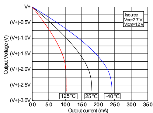
Figure 10. Positive output voltage swing vs output current V_{CC} = 2.7 V
