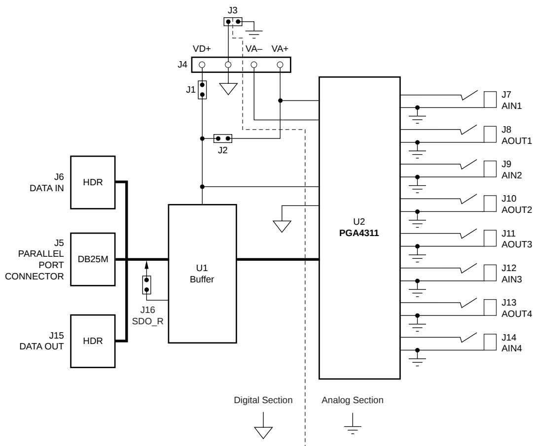
Figure 1. EVM Block Diagram.
