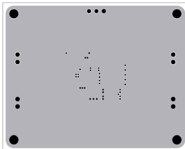
Figure 18. Demonstration Board, Second Layer
