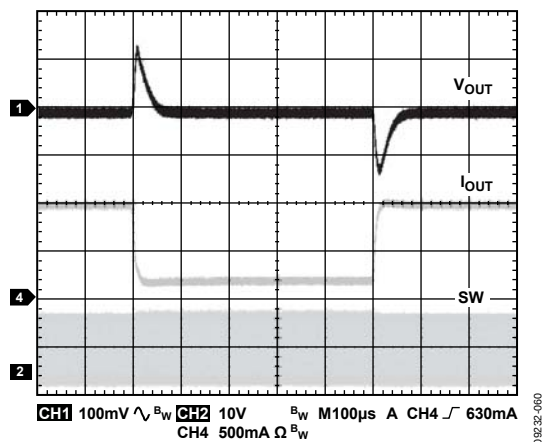
Figure 10. ADP2300 Load Transient, 0.2 A to 1.0 A, V_{OUT} = 3.3 V, V_{IN} = 12 V ( f_{SW} = 700 kHz, L = 10 µH, C_{OUT} = 22 µF)
