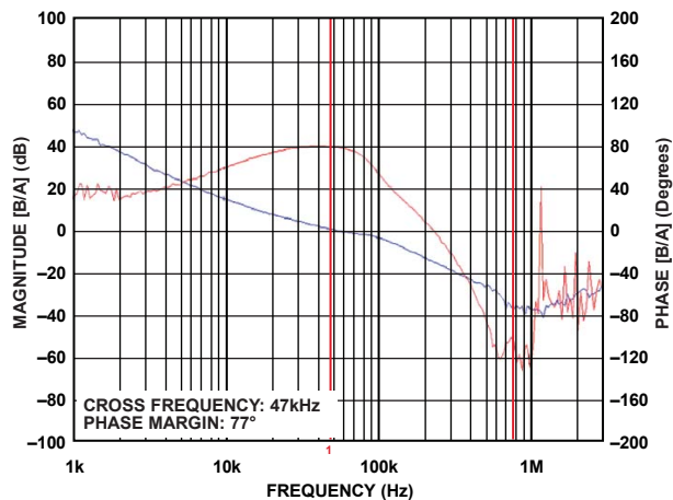
Figure 13. ADP2300 Bode Plot, V_{OUT} = 3.3 V, V_{IN} = 12 V ( f_{SW} = 700 kHz, L = 10 µH, C_{OUT} = 22 µF)
