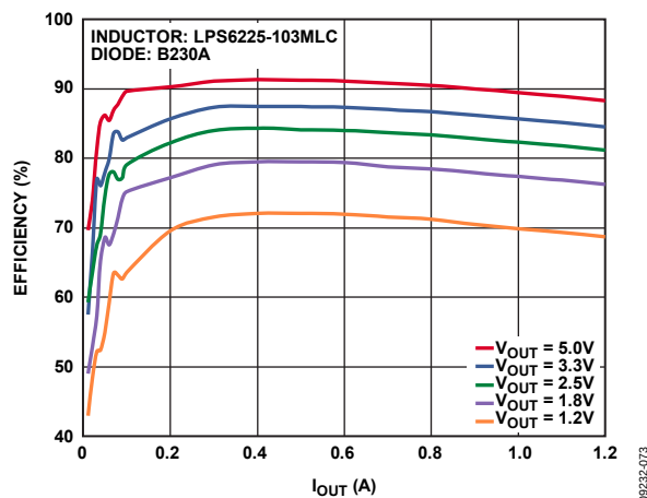
Figure 3. Efficiency Curve, V_{IN} = 12V , f_{SW} = 700kHz
