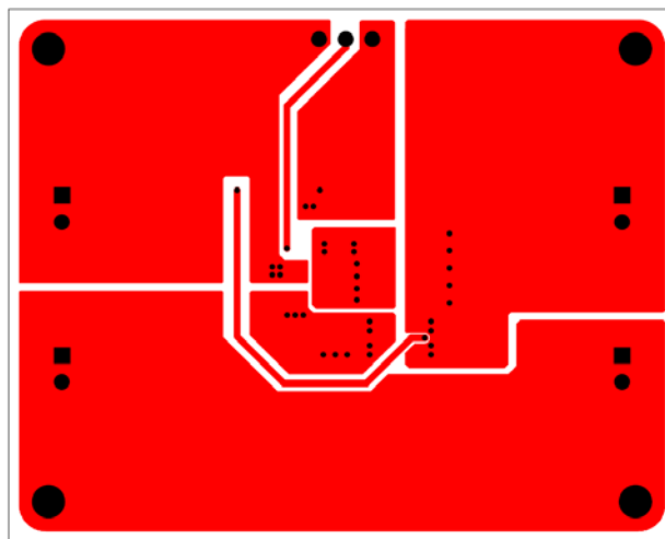
Figure 19. Demonstration Board, Bottom Layer
