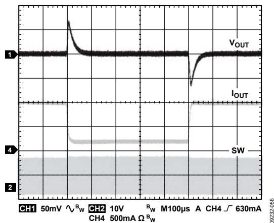
Figure 9. ADP2301 Load Transient, 0.2 A to 1.0 A, V_{OUT} = 3.3 V, V_{IN} = 12 V ( f_{SW} = 1.4 MHz, L = 4.7 µH, C_{OUT} = 22 µF)
