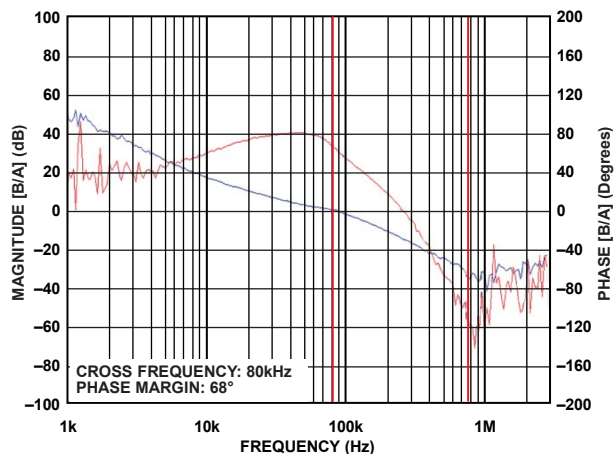
Figure 12. ADP2301 Bode Plot, V_{OUT} = 3.3 V, V_{IN} = 12 V ( f_{SW} = 1.4 MHz, L = 4.7 µH, C_{OUT} = 22 µF)
