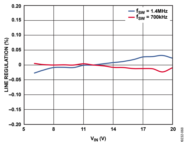
Figure 4. Line Regulation, V_{OUT} = 3.3V , I_{OUT} = 500mA
