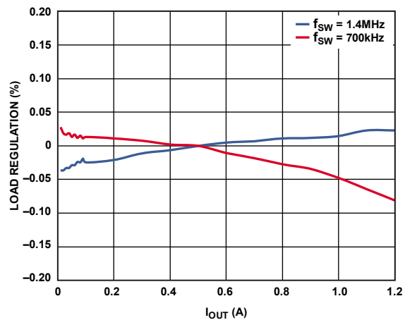
Figure 5. Load Regulation, V_{OUT} = 3.3V , V_{IN} = 12V
