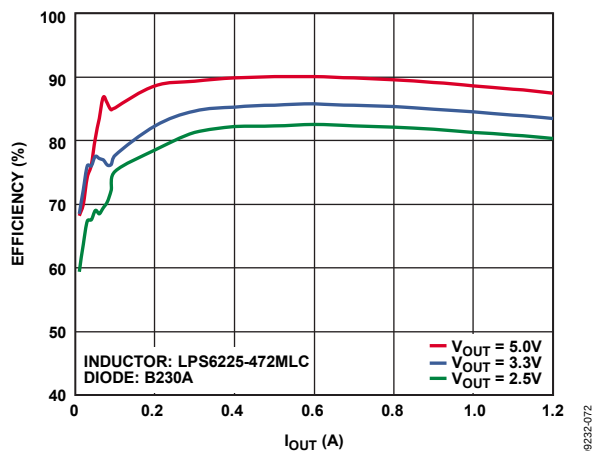
Figure 2. Efficiency Curve, V_{IN} = 12V , f_{SW} = 1.4MHz
