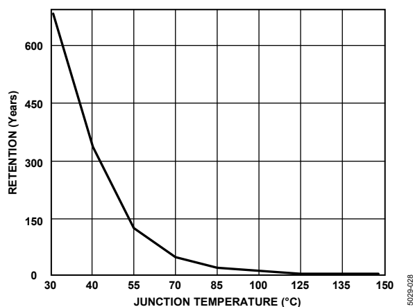
Figure 48. Flash Memory Retention
