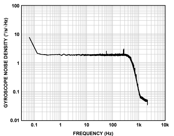
Figure 12. Gyroscope Noise Density, T_c = 25^\circ\text{C}
