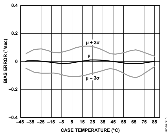
Figure 10. Gyroscope Bias Error, -40°C to +85°C, 1°C/min
