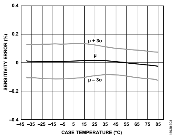
Figure 8. Gyroscope Sensitivity Error, -40°C to +85°C, 1°C/min
