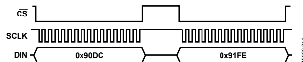
Figure 36. SPI Sequence for Writing 0xFEDC to XG_BIAS_LOW
