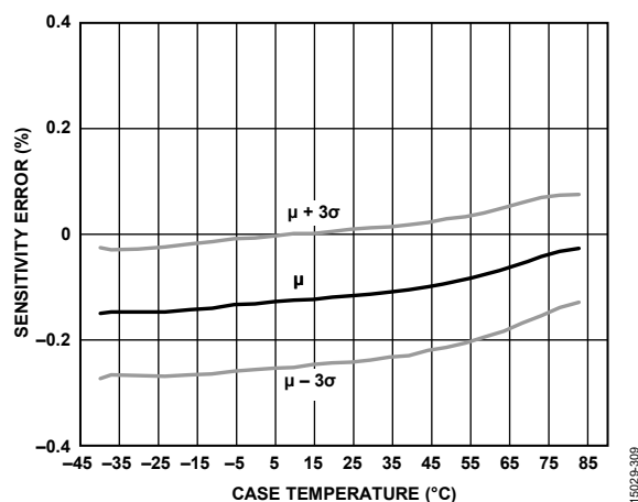
Figure 9. Gyroscope Sensitivity Error, +85°C to -40°C, 1°C/min
