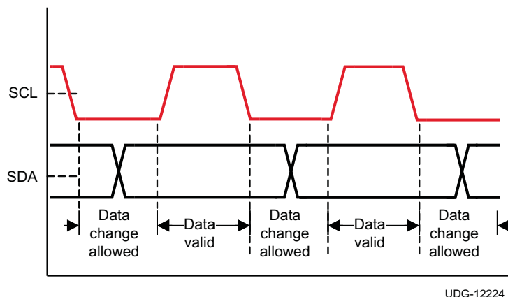
Figure 20. I 2 C Signals: Data Validity
