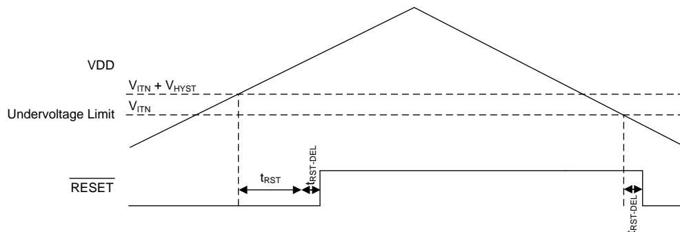
Figure 21. Undervoltage Detection
