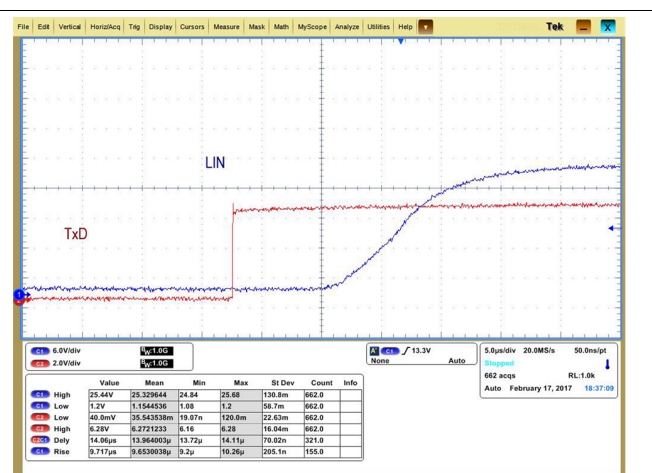
Figure 25. Dominant to Recessive Propagation
