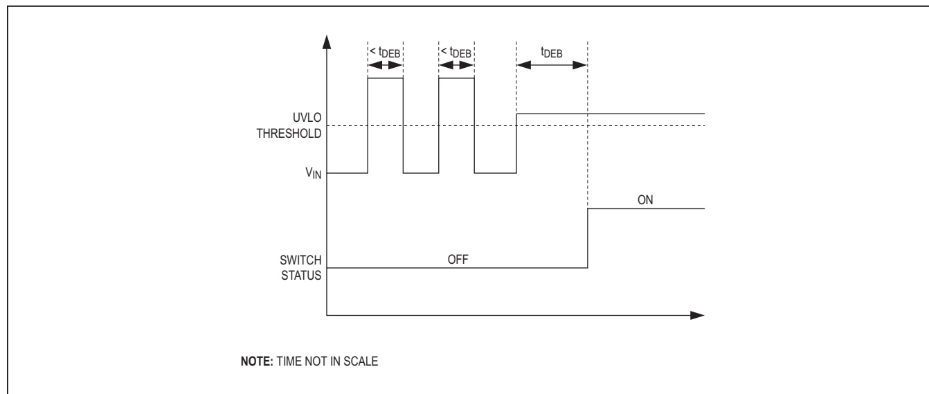
Figure 4. Debounce Timing
