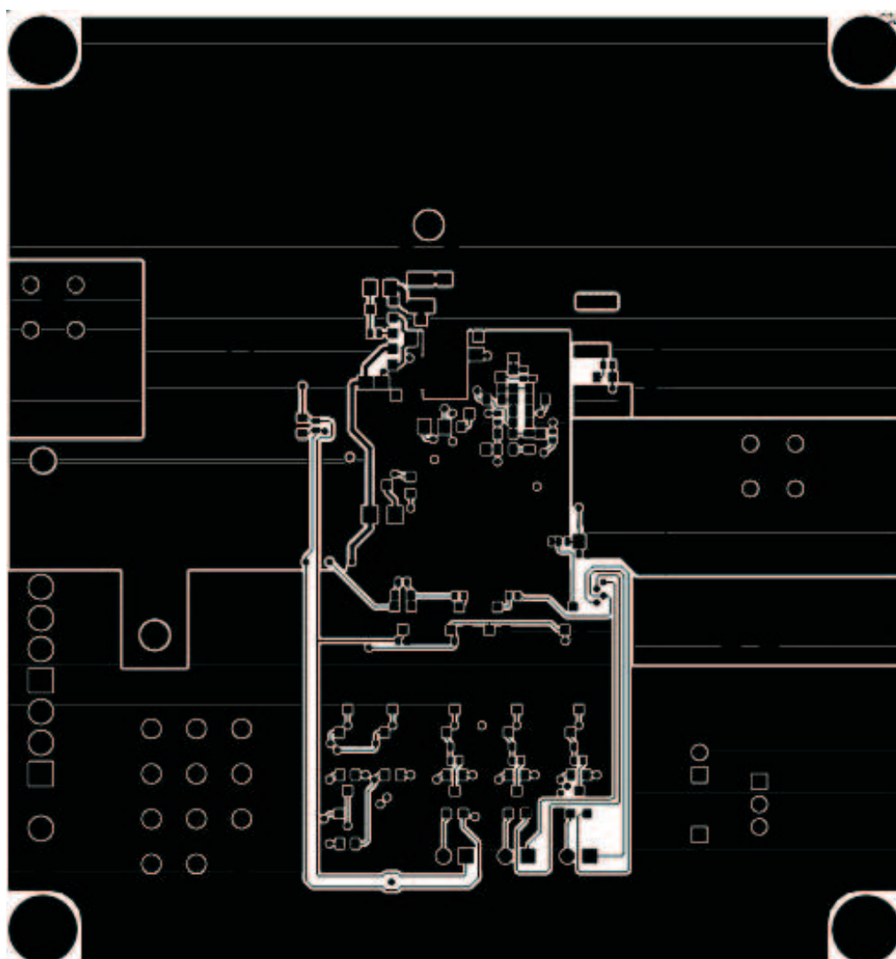
Figure 8. Bottom Layer
