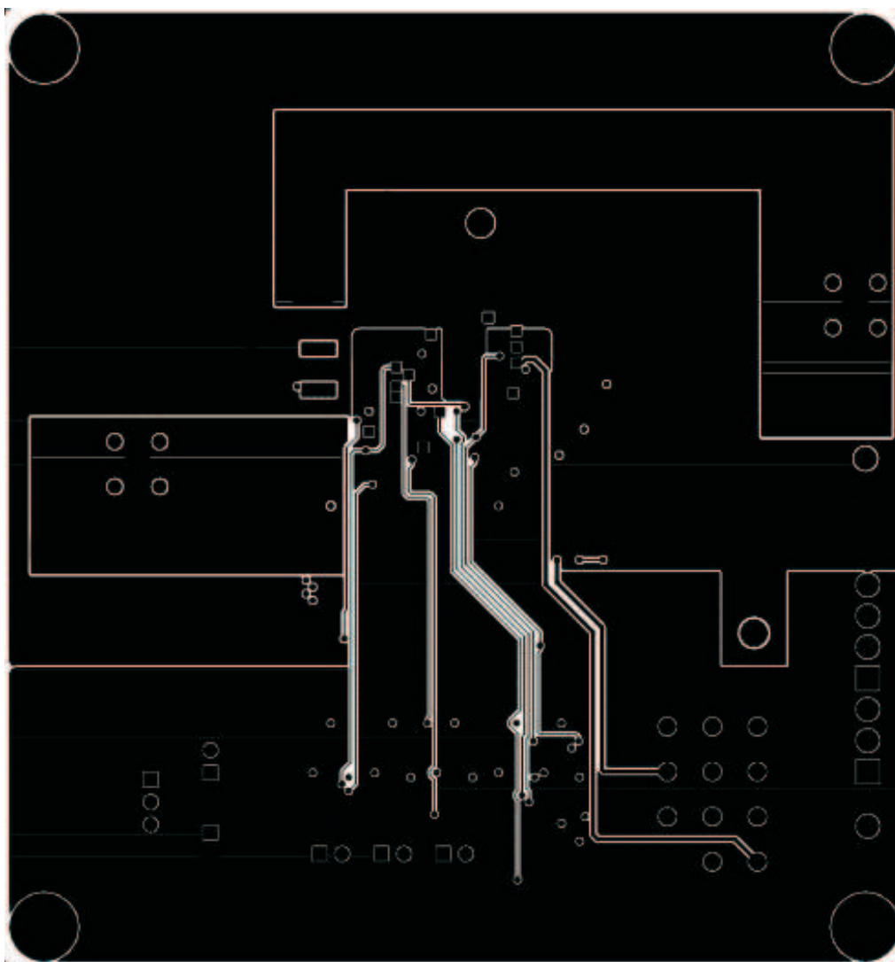
Figure 7. 3 rd Layer
