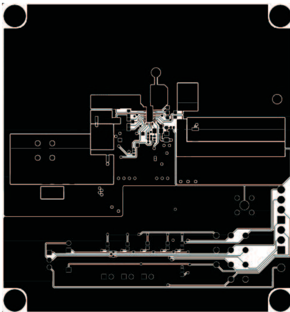
Figure 5. Top Layer
