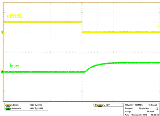
Figure 8. Current Ramp With a 16- \Omega , 1-mH, R_L Load and V_M = 8.2 V
