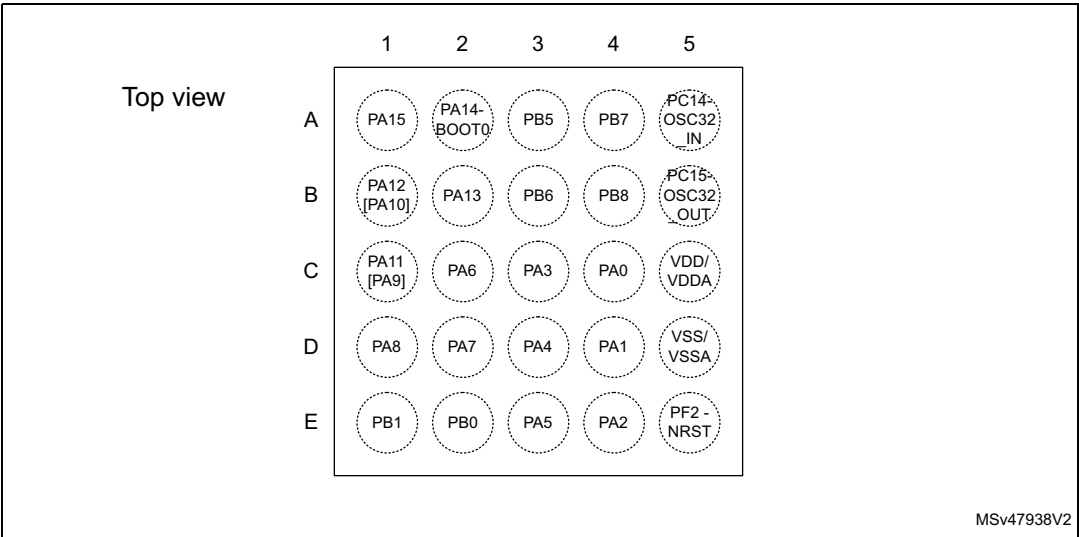
Figure 10. STM32G081Ex WLCSP25 pinout
