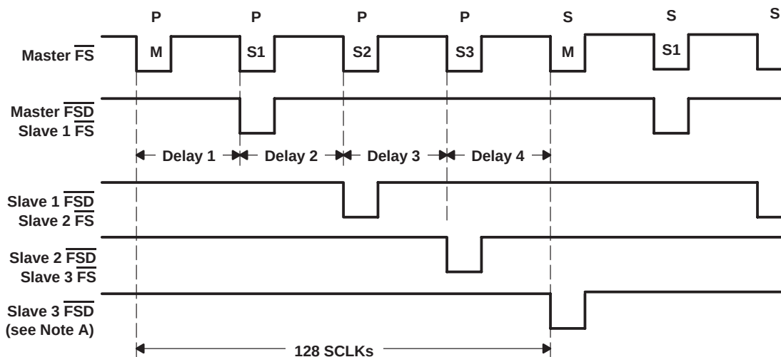
Figure 2–12. Master With Slaves (To DSP Interface)
