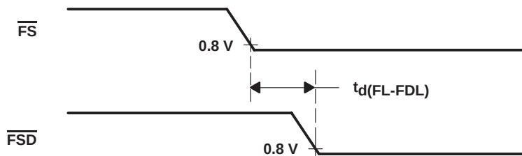
Figure 5–1. Master \overline{FS} and \overline{FSD} Timing
