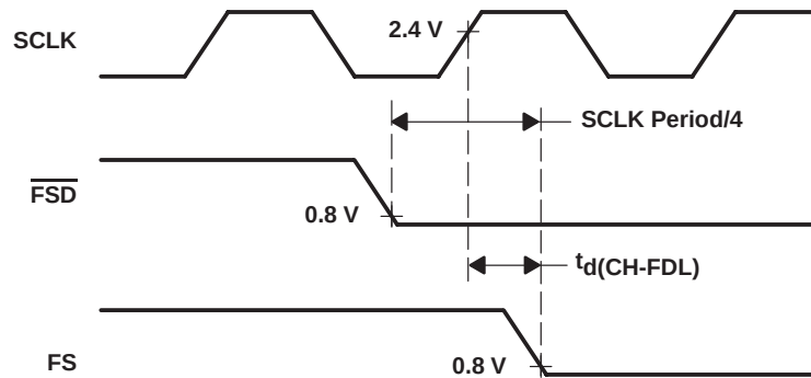
Figure 5–1. Master \overline{FS} and \overline{FSD} Timing
