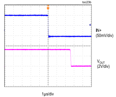
PROPAGATION DELAY t_{PD} ( V_{DD} = 3.3V )
