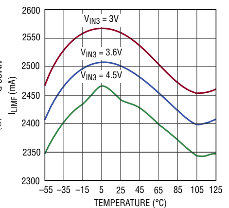
Buck-Boost Regulator Forward Current Limit
