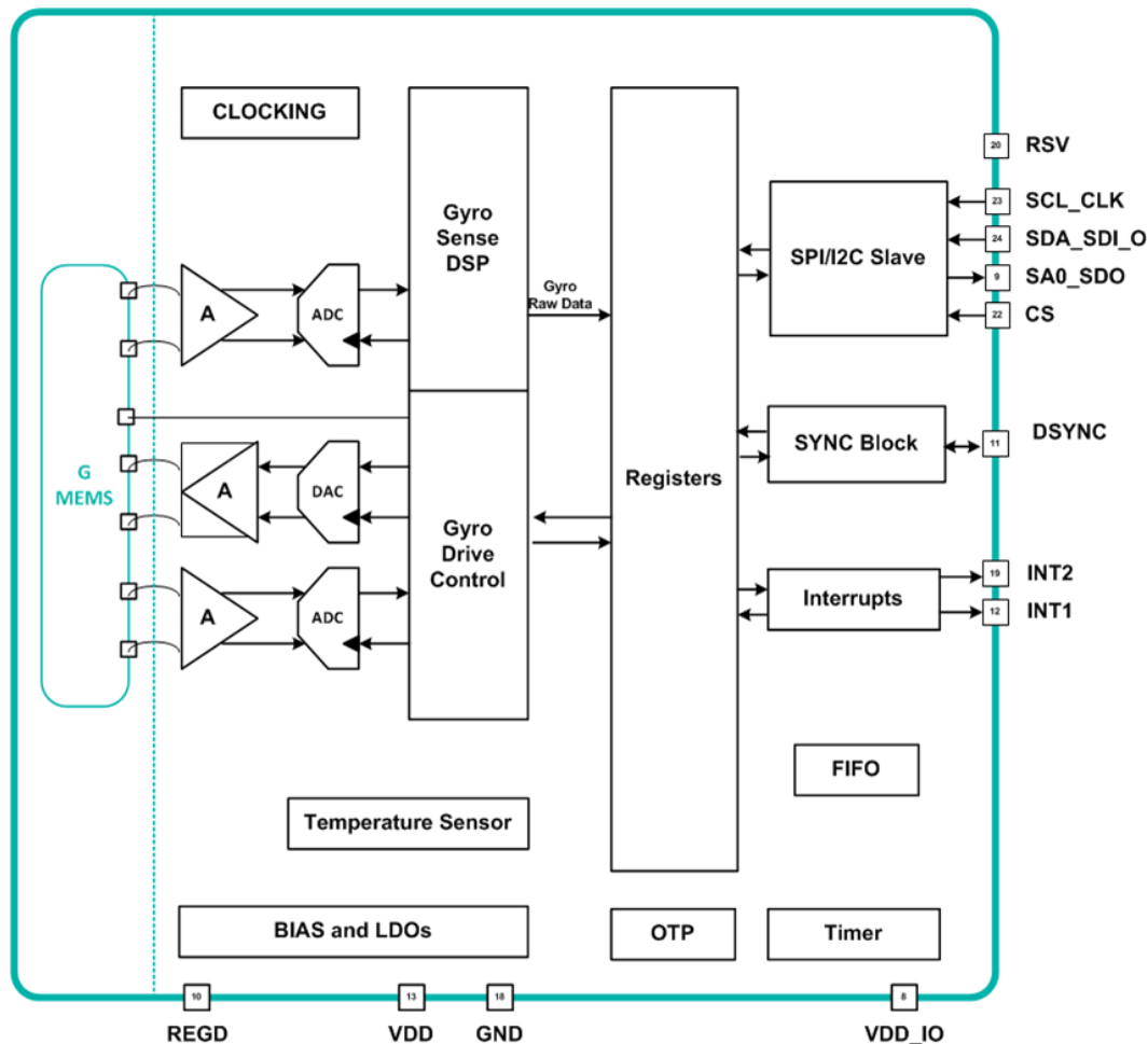
Figure 1: Block Diagram
