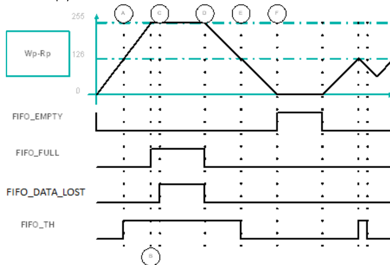
Figure 21: FIFO Flags
