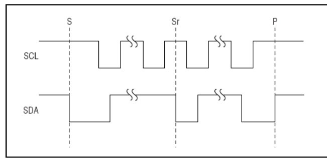
Figure 3: START (S), STOP (P), and Repeated START (Sr) Conditions
