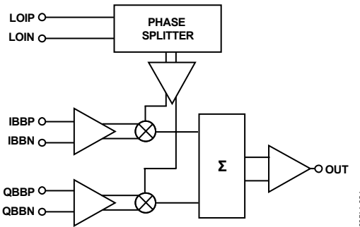
Figure 24. Block Diagram
