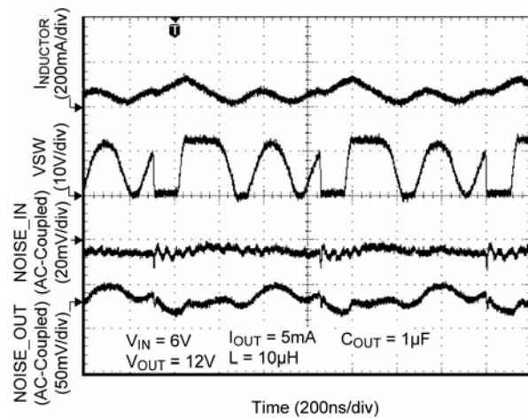
Switching Waveform - Discontinuous
