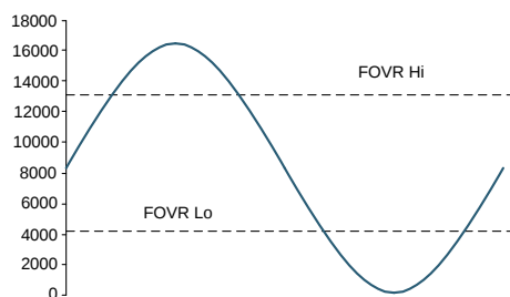
Figure 62. FOVR High and FOVR Low Thresholds
