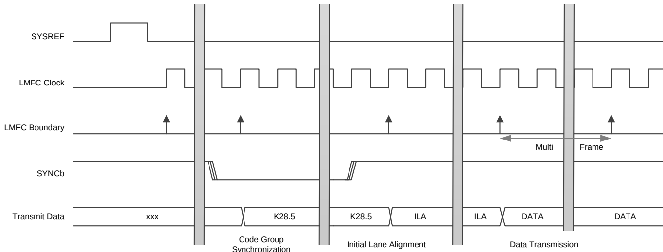
Figure 65. ILA Sequence
