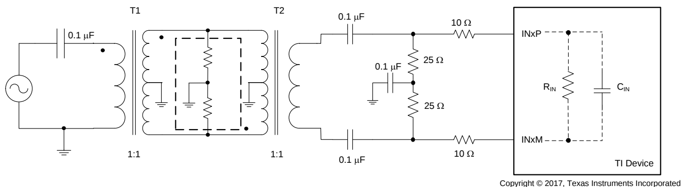
Figure 43. Analog Input Driving Circuit
