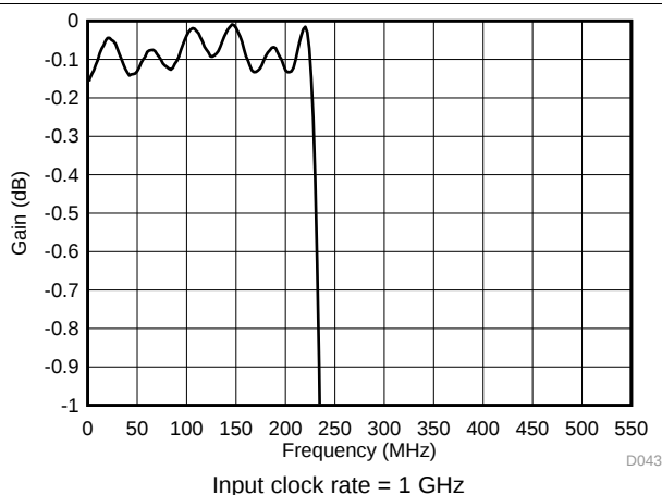
Figure 48. Decimation Filter Pass-Band Ripple vs Frequency
