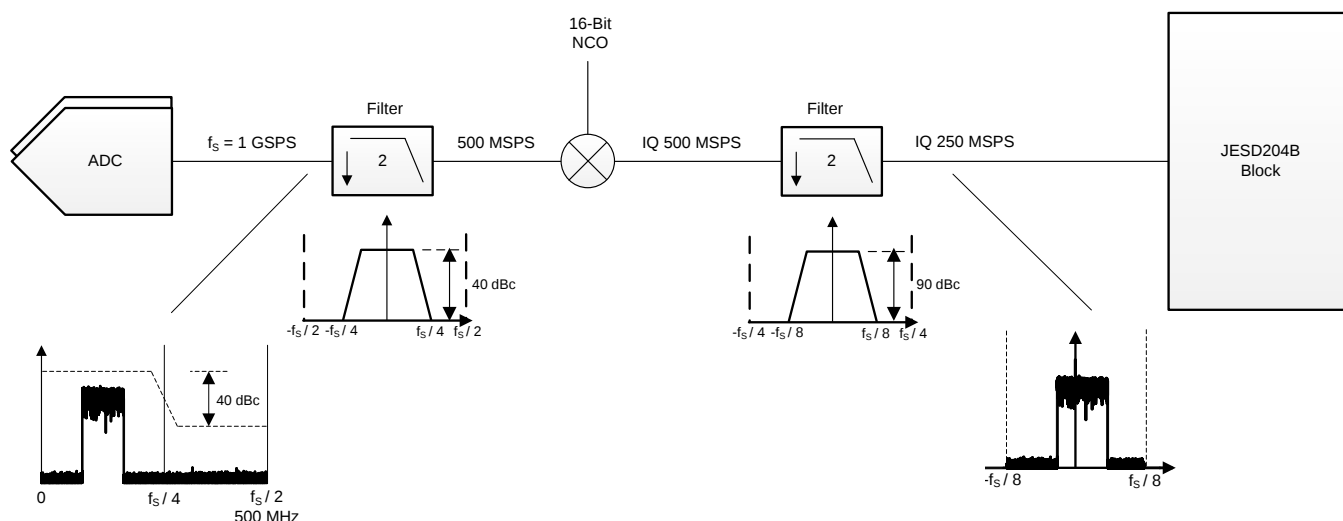
Figure 52. Operating Mode 1
