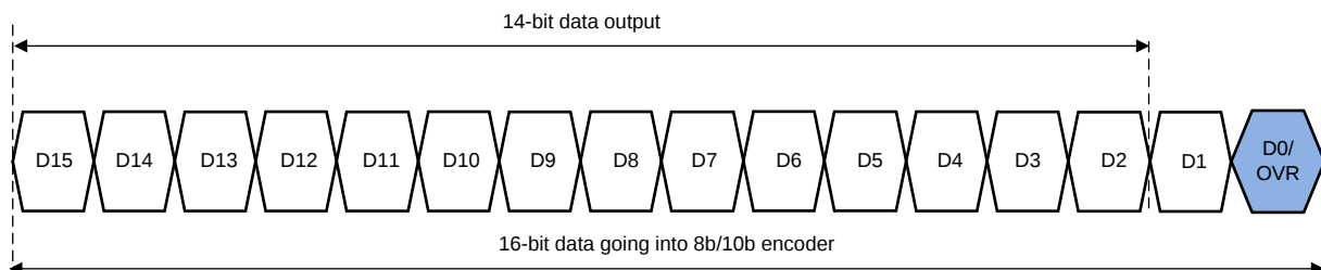
Figure 61. Timing Diagram for FOVR
