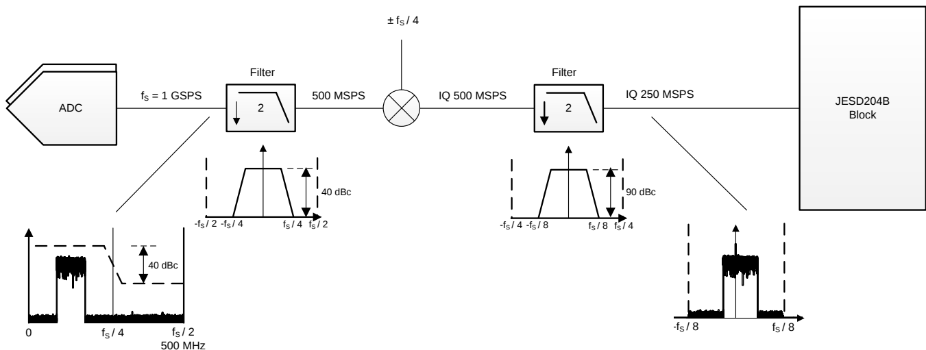
Figure 51. Operating Mode 0
