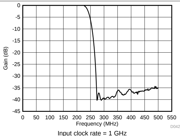
Figure 47. Decimation Filter Response vs Frequency
