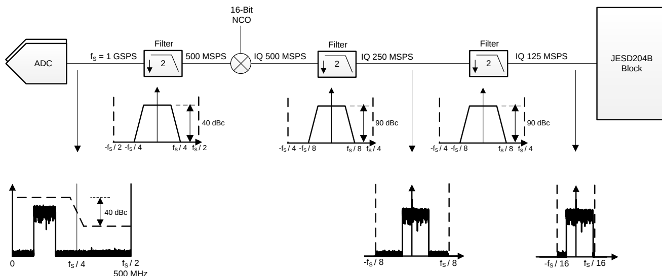
Figure 56. Operating Mode 6
