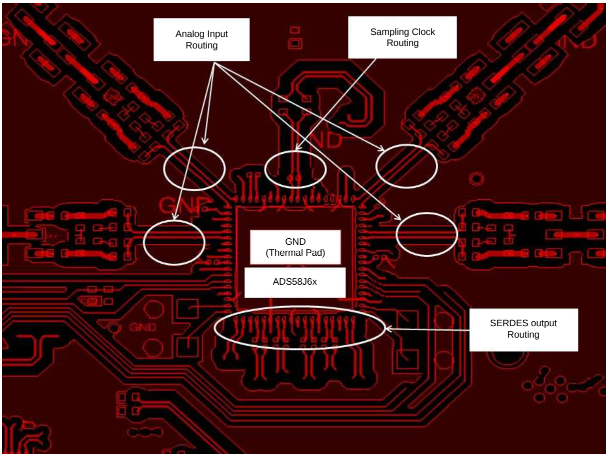
Figure 138. ADS58J64EVM Layout
