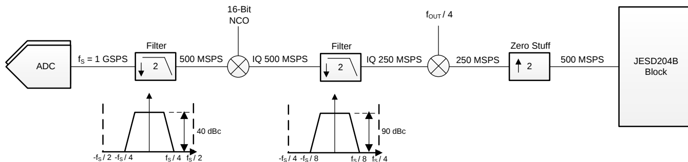
Figure 57. Operating Mode 7
