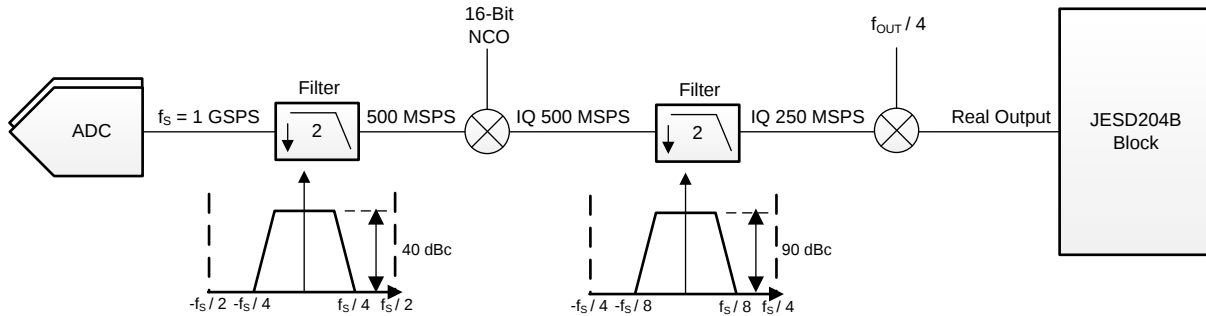
Figure 55. Operating Mode 4
