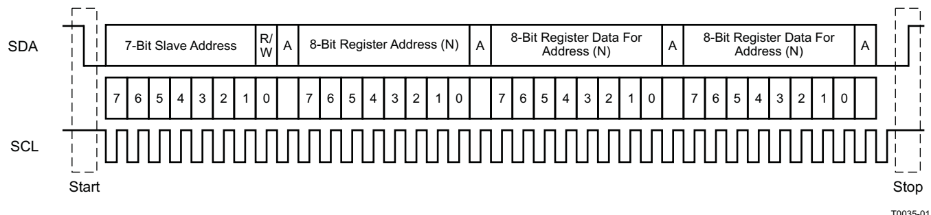
Figure 13. Typical I²C Sequence
