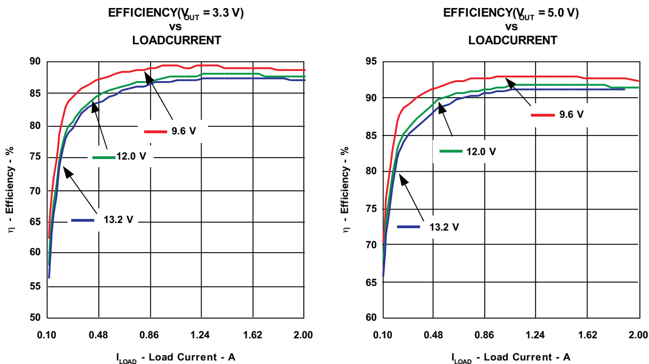
Figure 5. TPS54386EVM Efficiency verse Load Current V_{IN} = 9.6-13.2 V , V_{OUT1} = 5.0 V I_{OUT1} = 0-2 A , V_{OUT2} = 3.3 V I_{OUT2} = 0-2 A
