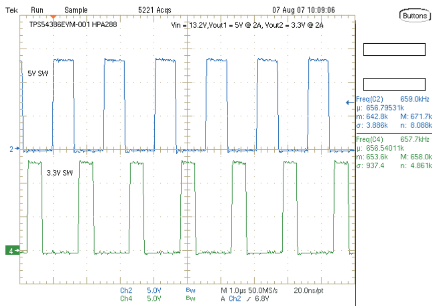
Figure 8. TPS54386EVM Switching Waveforms V_{IN} = 12\text{ V} , I_{OUT} = 2\text{ A} Ch1: TP9 (SW1), Ch2: TP12 (SW2)
