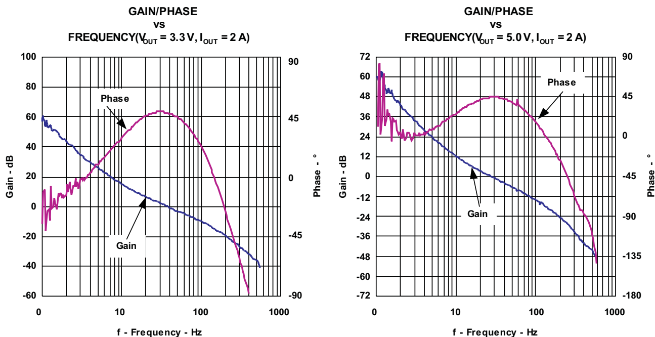
Figure 9. TPS54386EVM Gain and Phase vs Frequency
