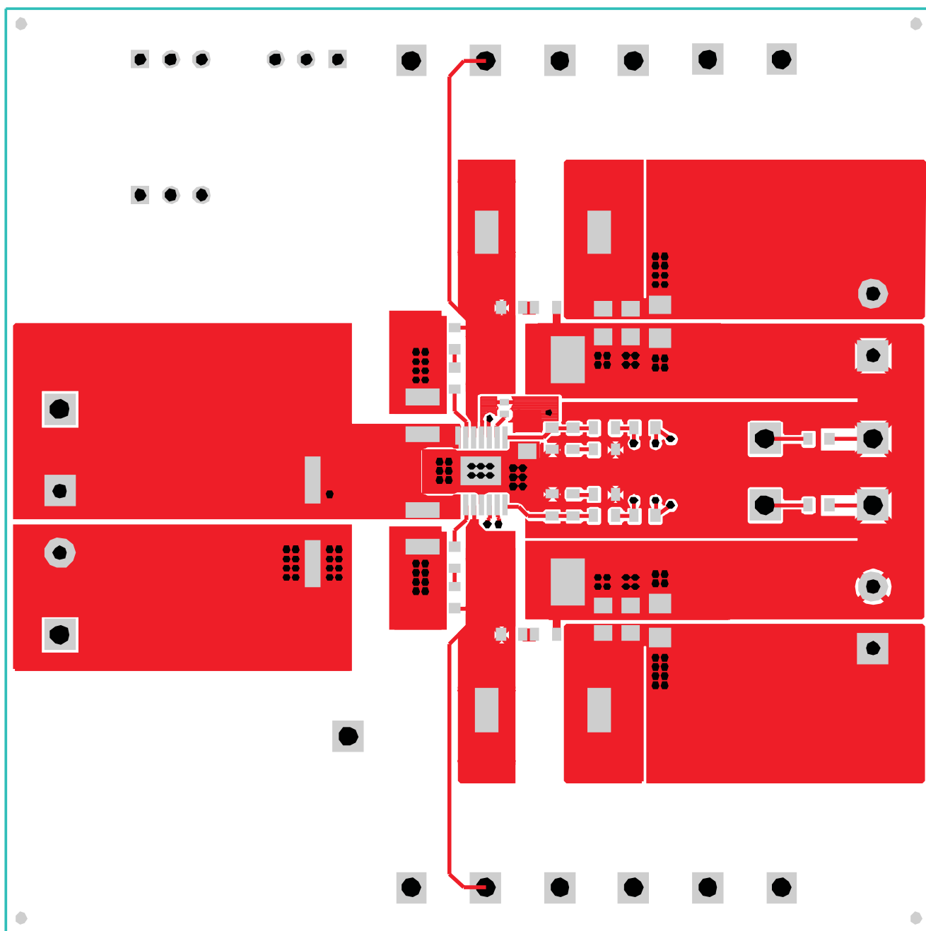
Figure 11. TPS54386EVM Top Copper (viewed from top)
