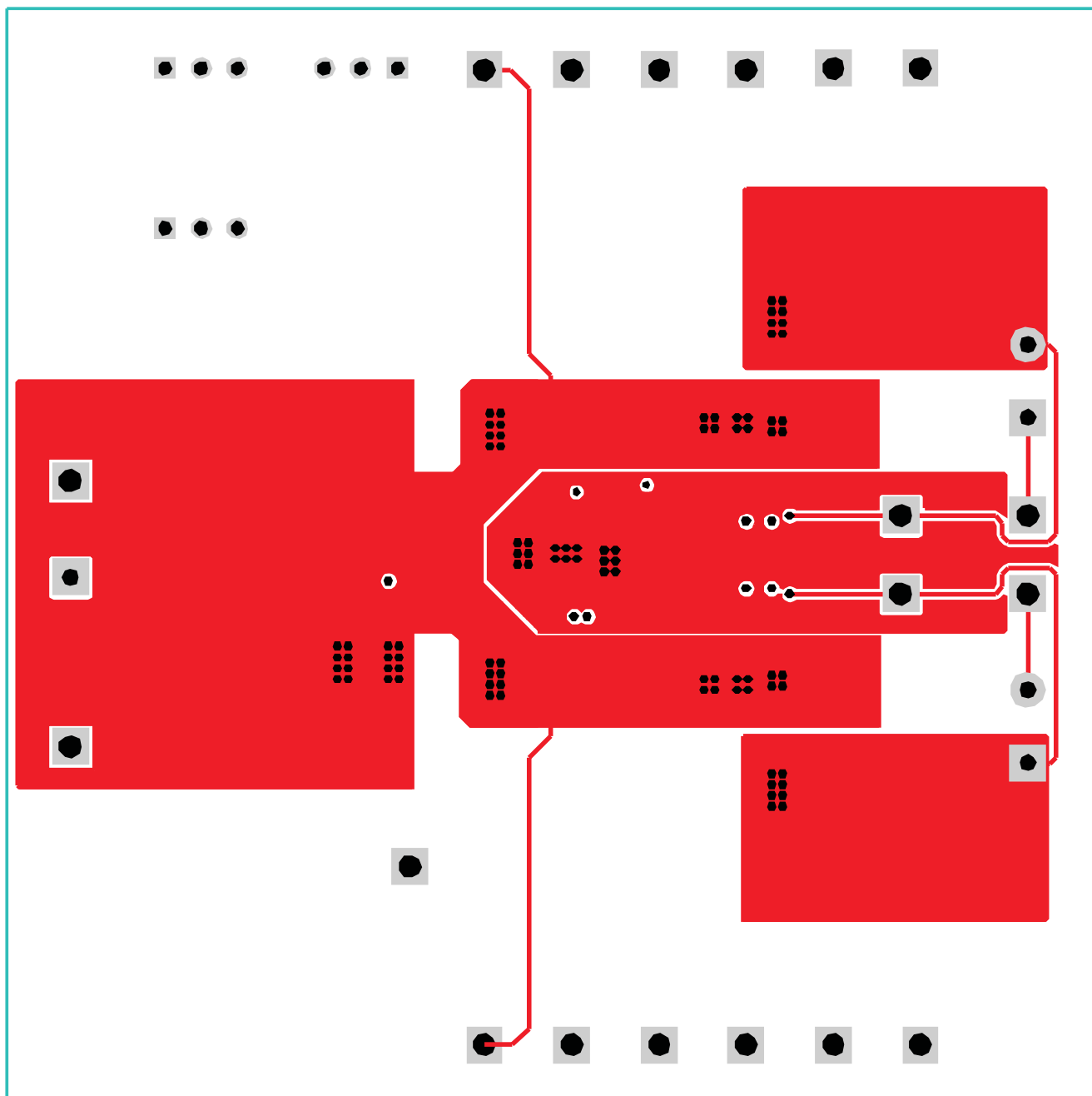
Figure 12. TPS54386EVM Bottom Copper (x-ray view from top)
