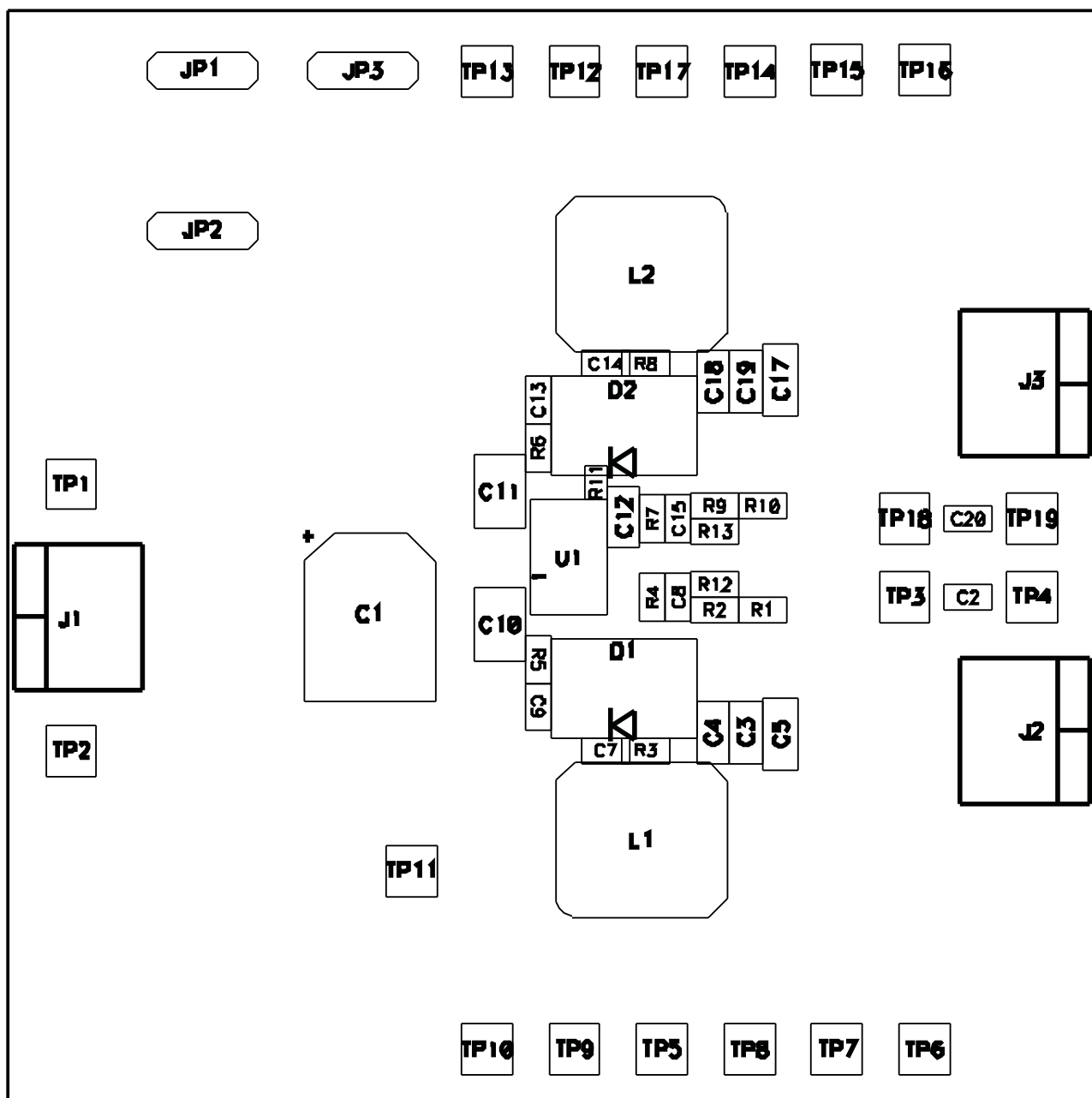
Figure 10. TPS54386EVM Component Placement (viewed from top)
