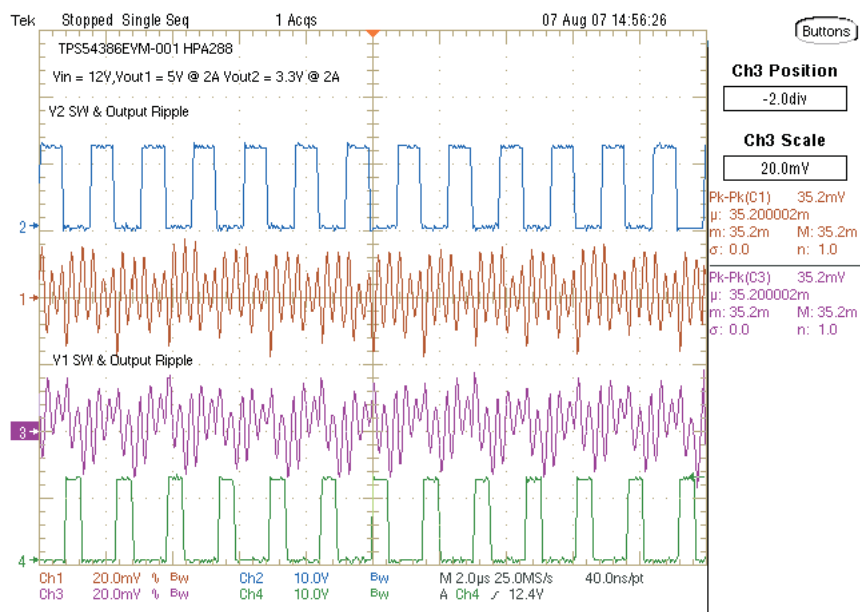
Figure 7. TPS54386EVM Output Voltage Ripple ( V_{IN} = 13.2 \text{ V} , I_{OUT1} = I_{OUT2} = 2 \text{ A} )
