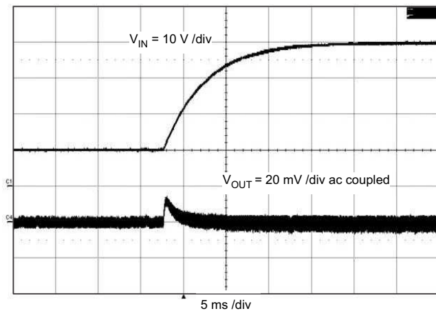
Figure 29. Line Transient
