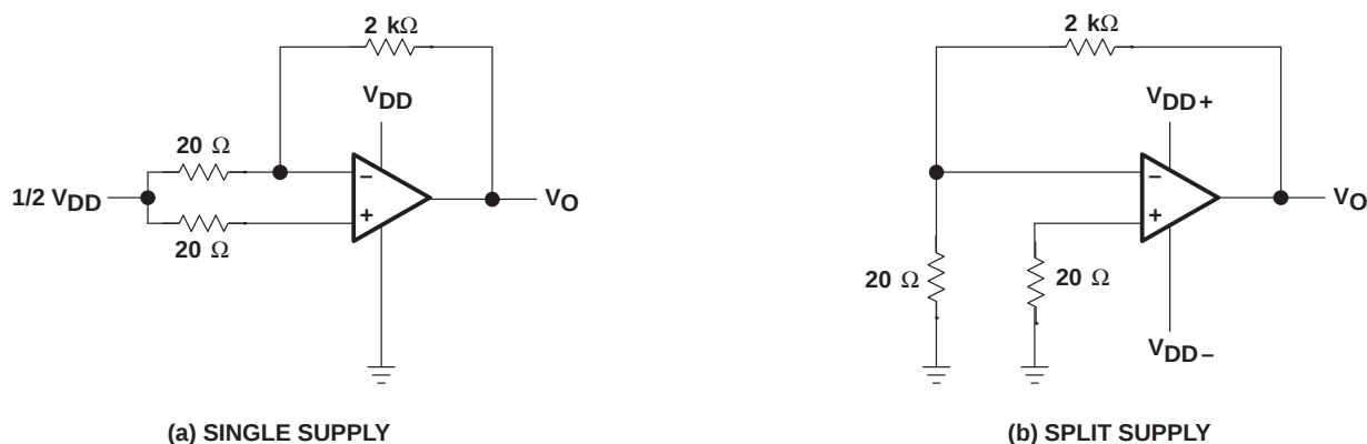
Figure 35. Noise-Test Circuit
