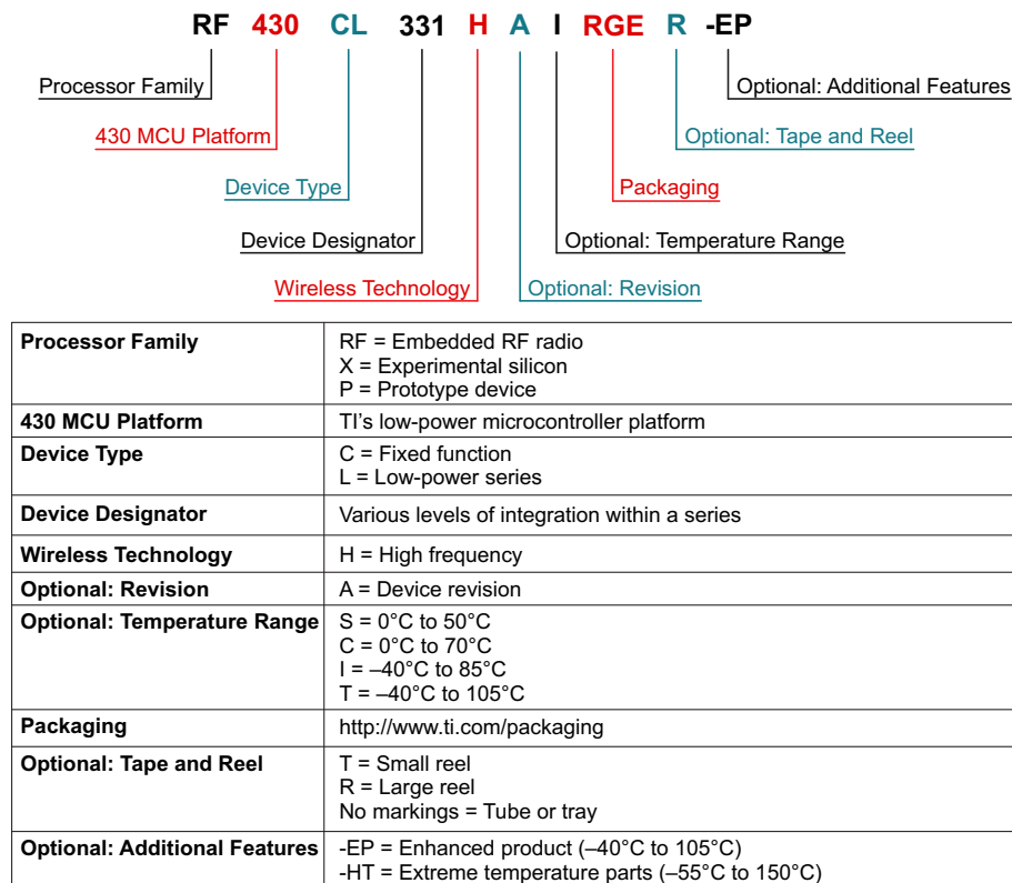
Figure 7-1. Device Nomenclature
