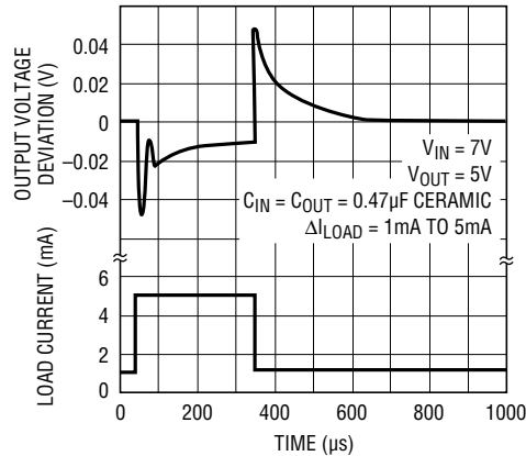
Transient Response
