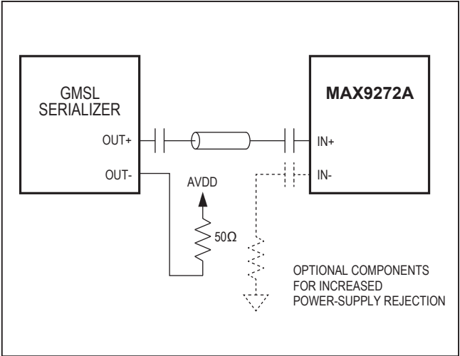
Figure 30. Coax-Mode Connection Diagram
