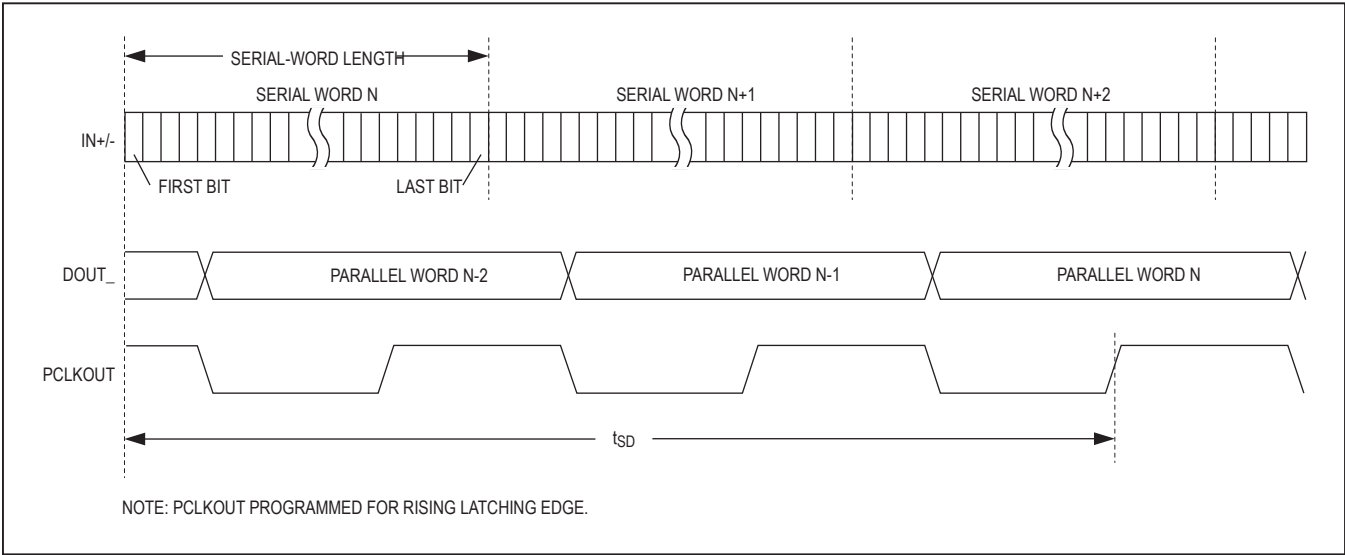
Figure 7. Deserializer Delay
