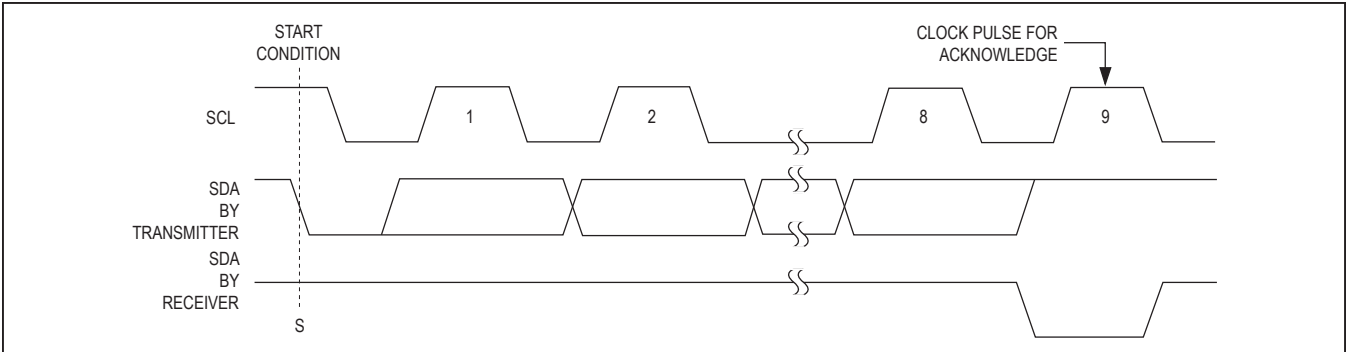
Figure 24. Acknowledge
