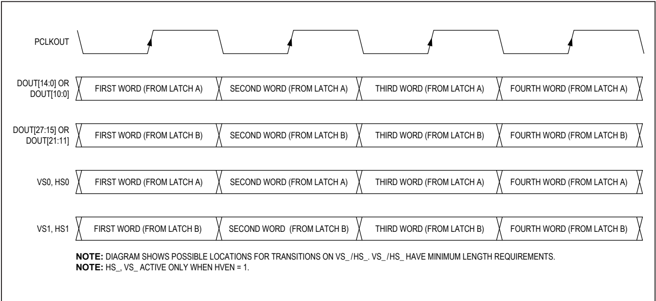
Figure 12. Single-Output Waveform (Serializer Using Double Input)
