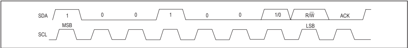
Figure 25. Slave Address
