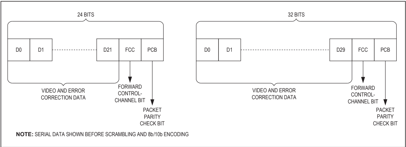
Figure 15. Serial-Data Format
