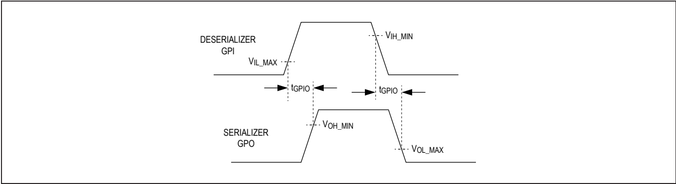
Figure 8. GPI-to-GPO Delay
