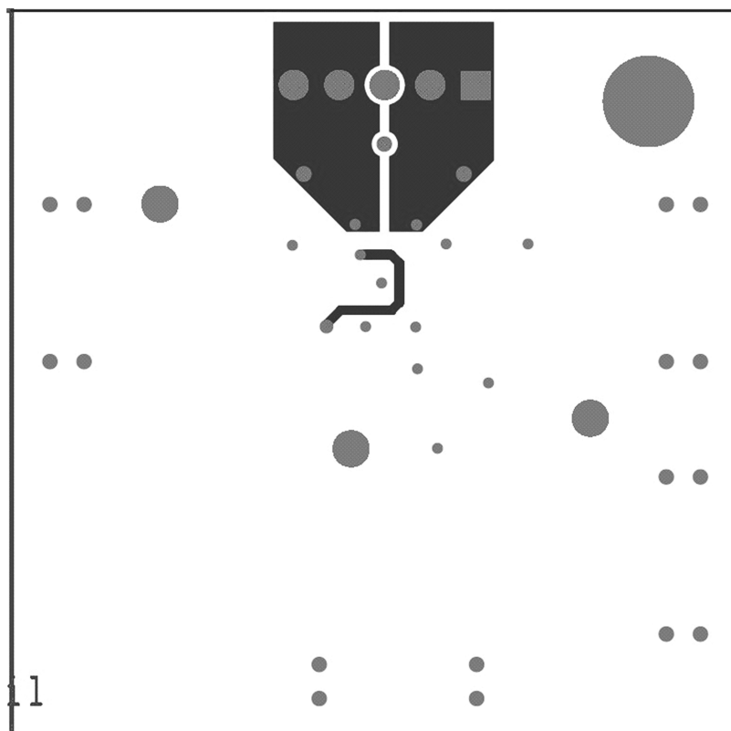
Figure 4. Evaluation Board Layer 2 (bottom view)
