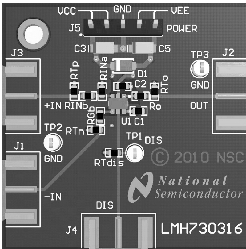
Figure 2. Evaluation Board Top Layer
