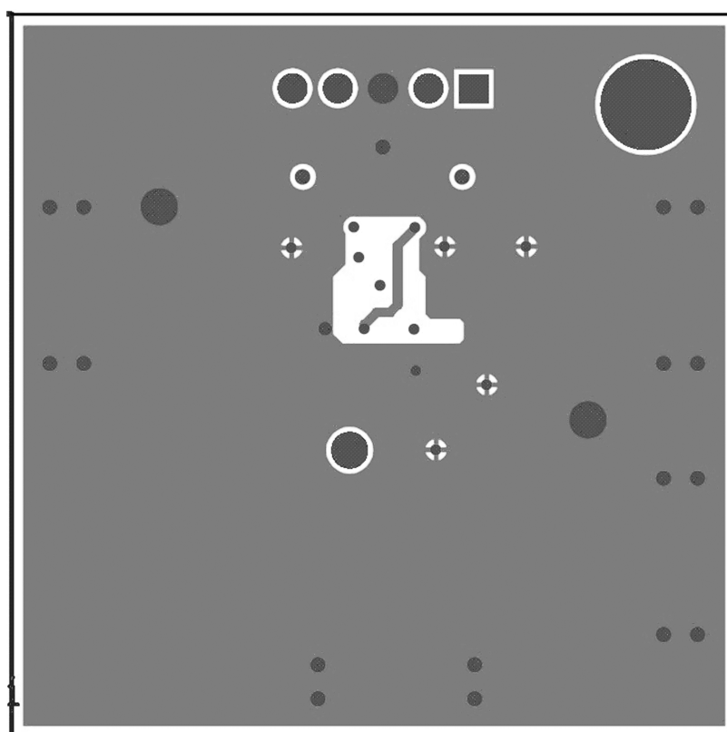
Figure 5. Evaluation Board Layer 3 (bottom view)
