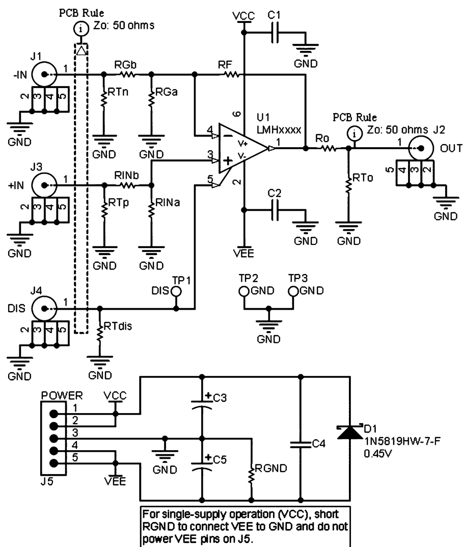
Figure 1. Evaluation Board Schematic
