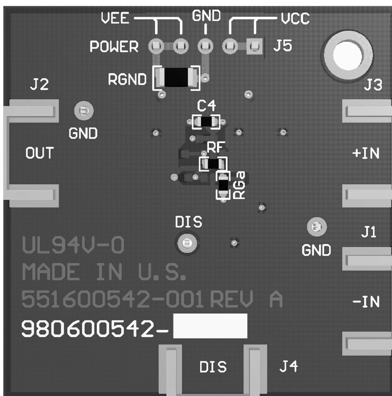
Figure 3. Evaluation Board Bottom Layer (bottom view)
