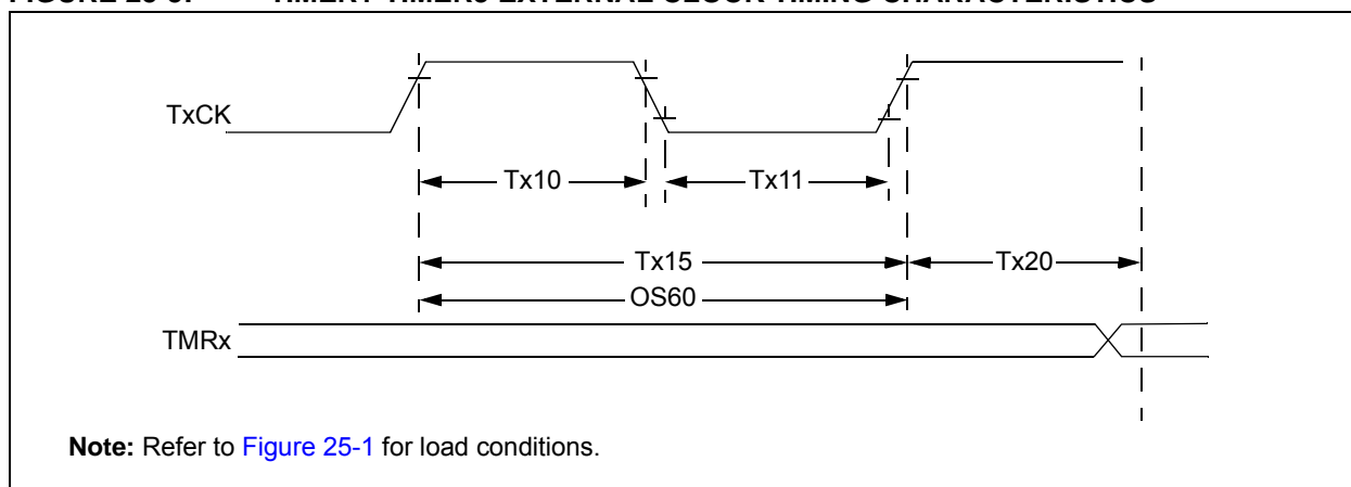
FIGURE 25-5: TIMER1-TIMER3 EXTERNAL CLOCK TIMING CHARACTERISTICS
