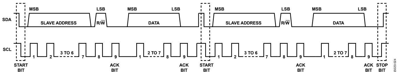
Figure 25. PC Repeated Start Sequence
