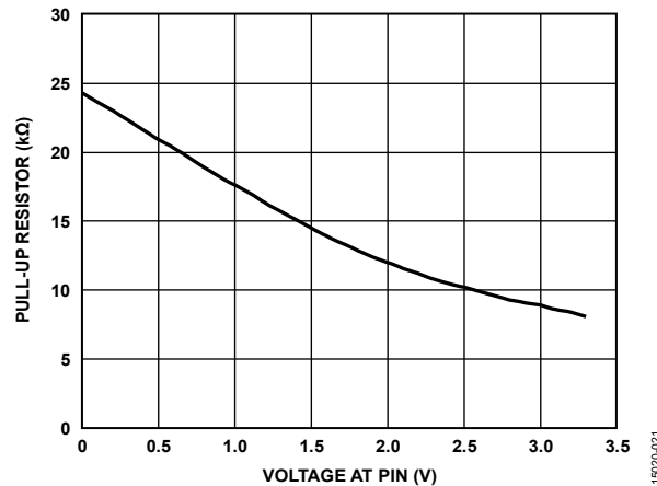
Figure 22. GPIO Pull-Up Resistor Value
