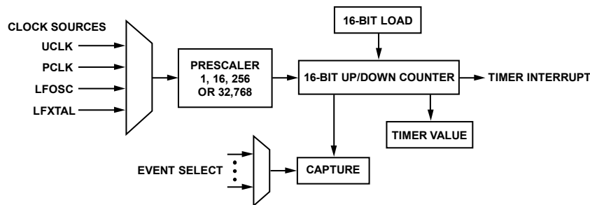
Figure 31. General-Purpose Timers Block Diagram
