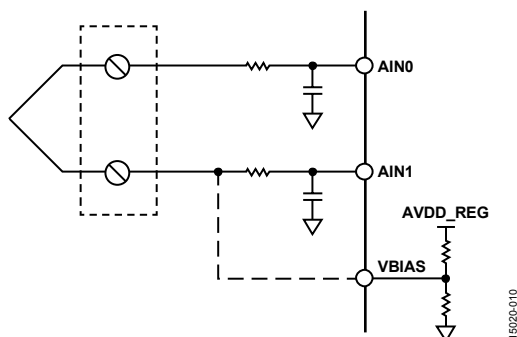
Figure 11. Using V_{BIAS} Voltage to Set Thermocouple Common-Mode Voltage
