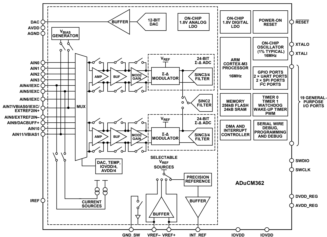
Figure 1. ADuCM362 Block Diagram
