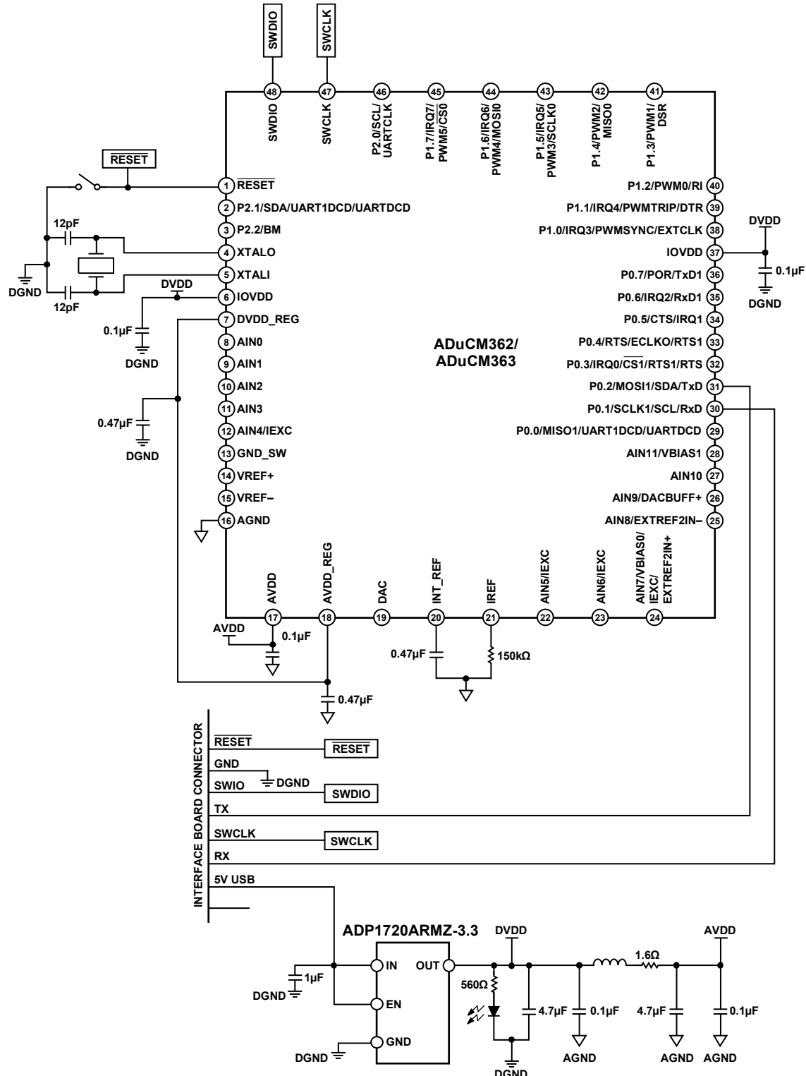
Figure 40. Typical System Configuration
