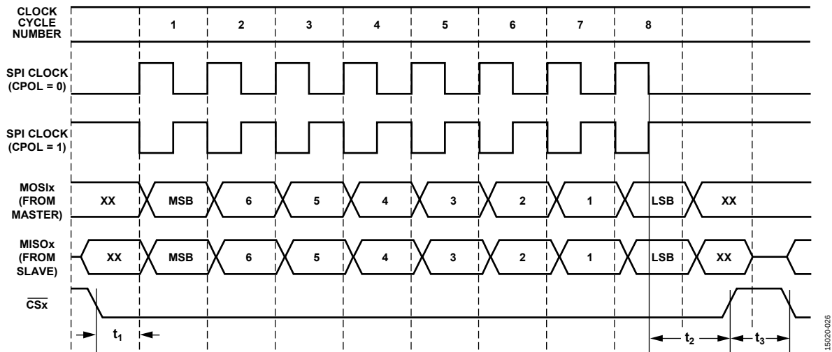
Figure 28. SPI Transfer Protocol, CPHA = 1
