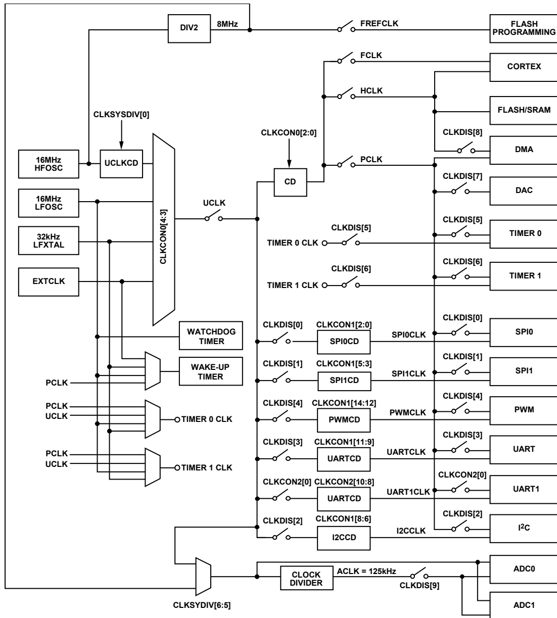
Figure 4. ADuCM362 Clocking Architecture Block Diagram (the ADuCM363 Clocking Architecture Block Diagram is Identical, Except ADC0 Is Removed)
