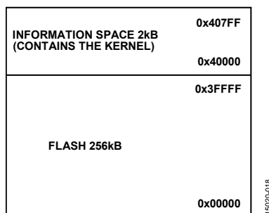
Figure 19. Information and User Space Memory Map on the ADuCM362/ADuCM363
