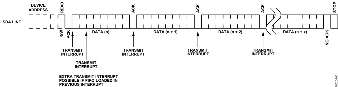
Figure 26. I²C Slave Tx Interrupt Details
