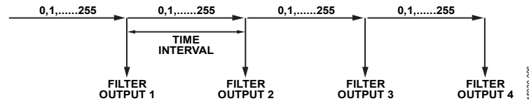
Figure 7. ADuCM362/ADuCM363 Step Detection Timing Diagram
