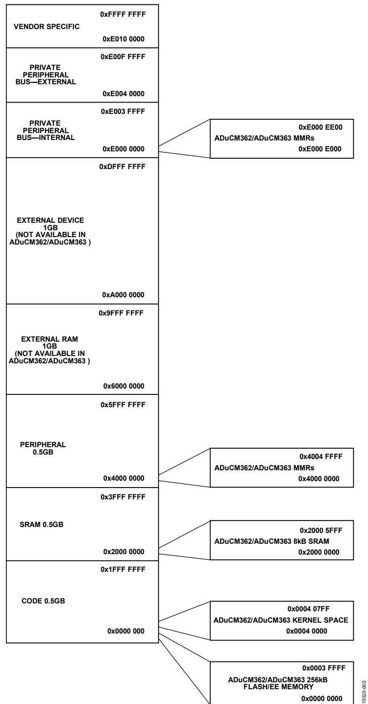
Figure 3. ADuCM362/ADuCM363 Cortex-M3 Memory Map Diagram Rev. A | Page 8 of 175
