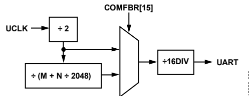
Figure 30. Baud Rate Generation
