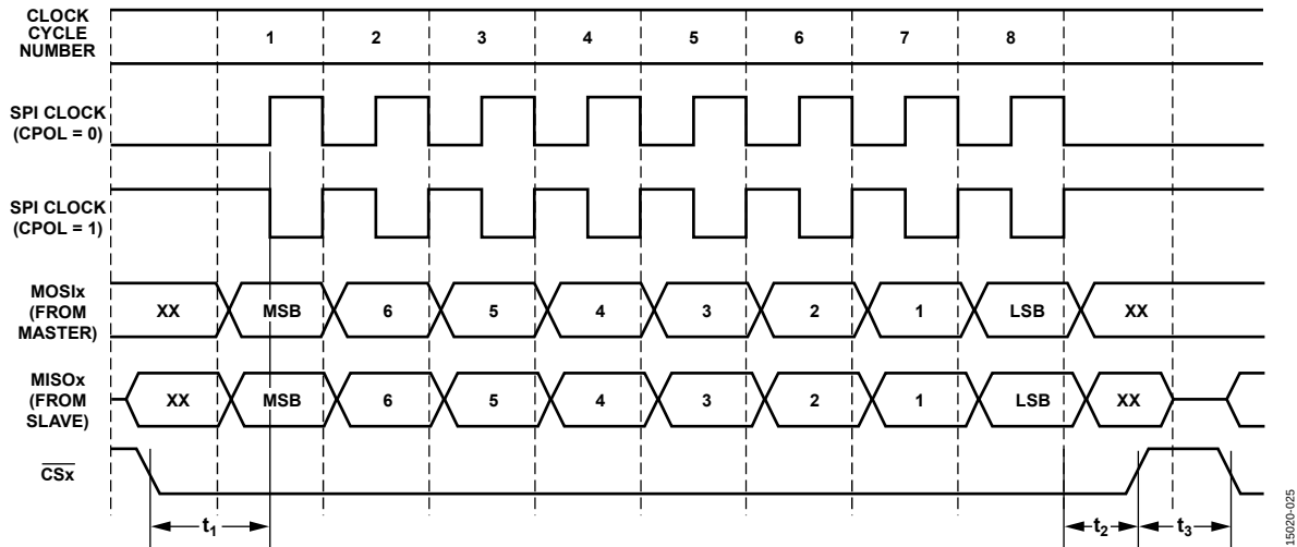
Figure 27. SPI Transfer Protocol, CPHA = 0
