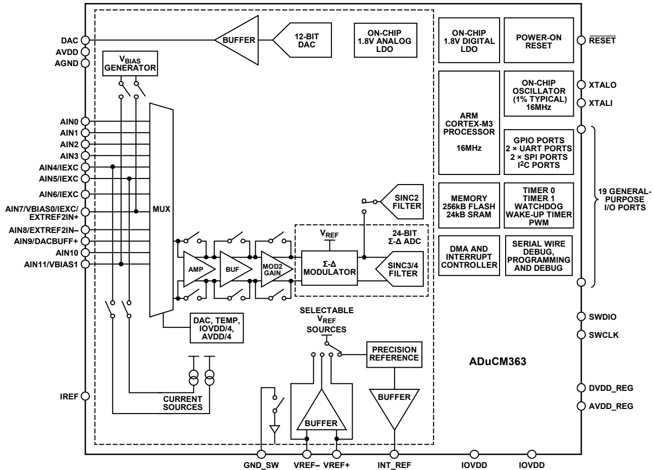
Figure 2. ADuCM363 Block Diagram
