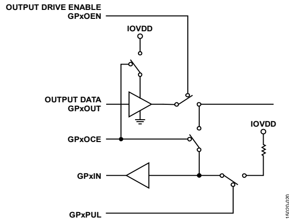
Figure 21. GPIO Structure
