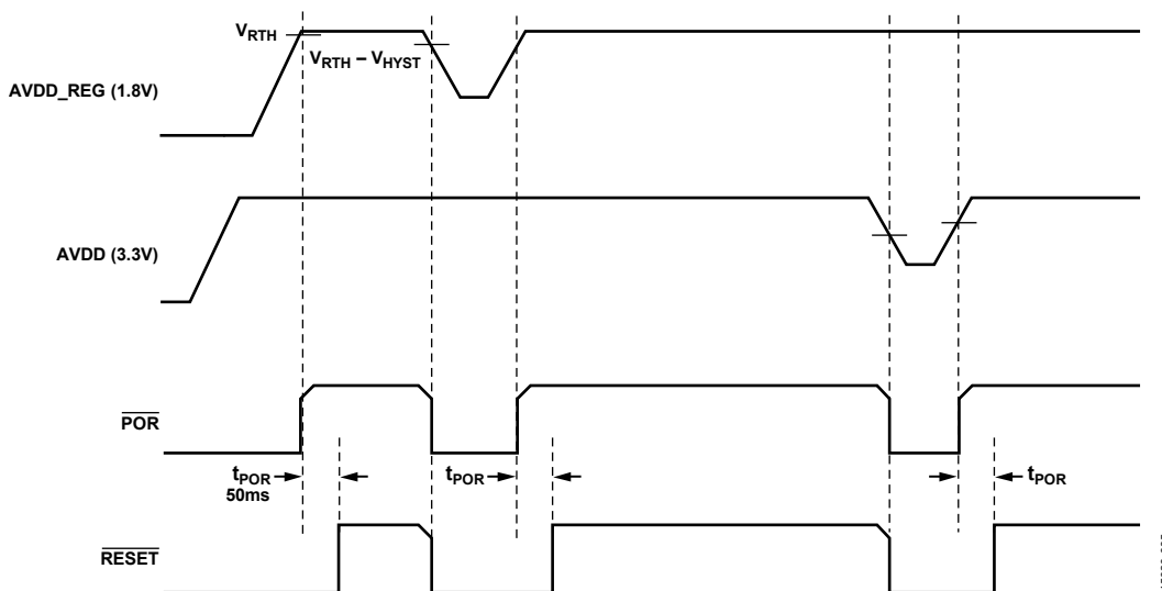
Figure 38. Typical Power-On Cycle
