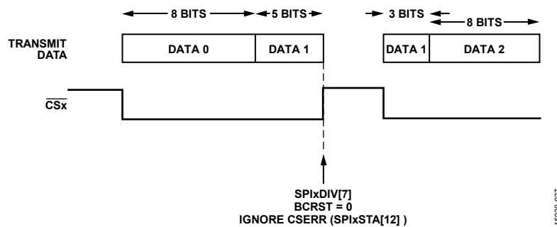
Figure 29. SPI Communication: Midbyte Stall
