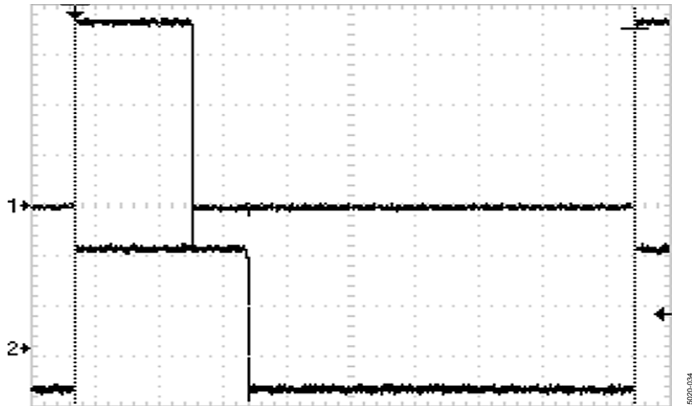
Figure 36. PWM Output on the PWM0 and PWM1 Pins Generated by the Previously Described Code; PWM0 is Channel 2
