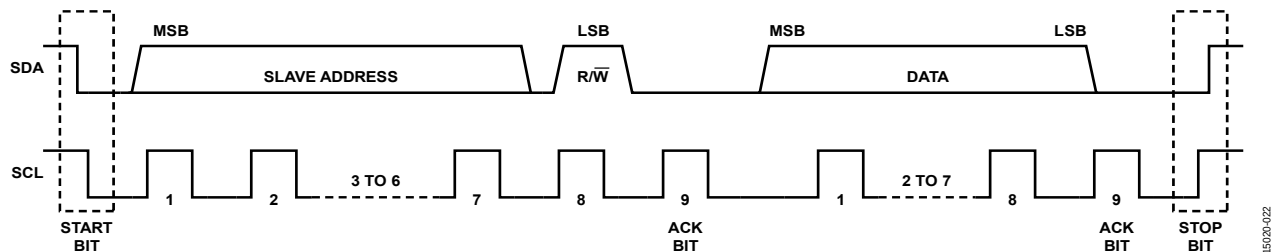
Figure 23. Typical I 2 C Transfer Sequence
