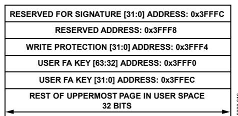
Figure 20. Uppermost Page of User Memory
