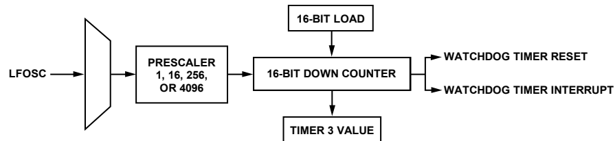
Figure 34. Watchdog Timer Block Diagram
