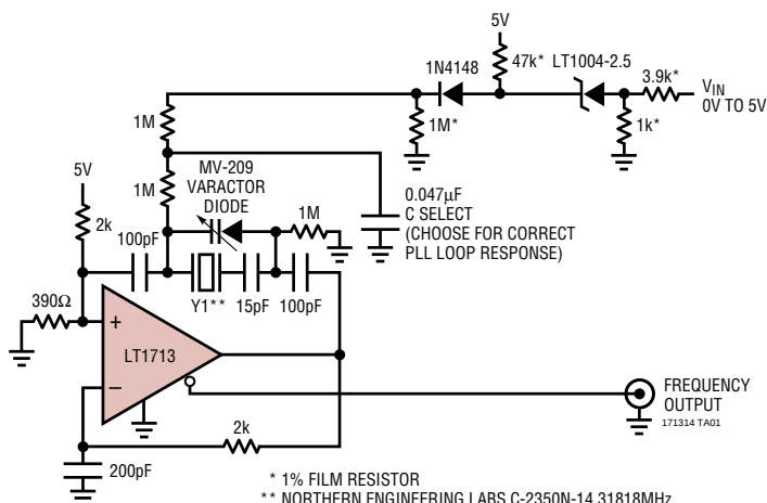
A 4× NTSC Subcarrier Voltage-Tunable Crystal Oscillator
