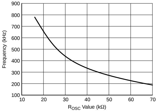
Figure 4. Oscillator Frequency vs. R_{OSC} Value
