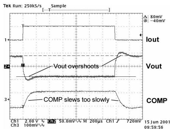
Figure 23. The Value of C_{AMP} Is Too High and the Loop Gain/Bandwidth Too Low. COMP Slews Too Slowly Which Results in Overshoot in V_{OUT} .
