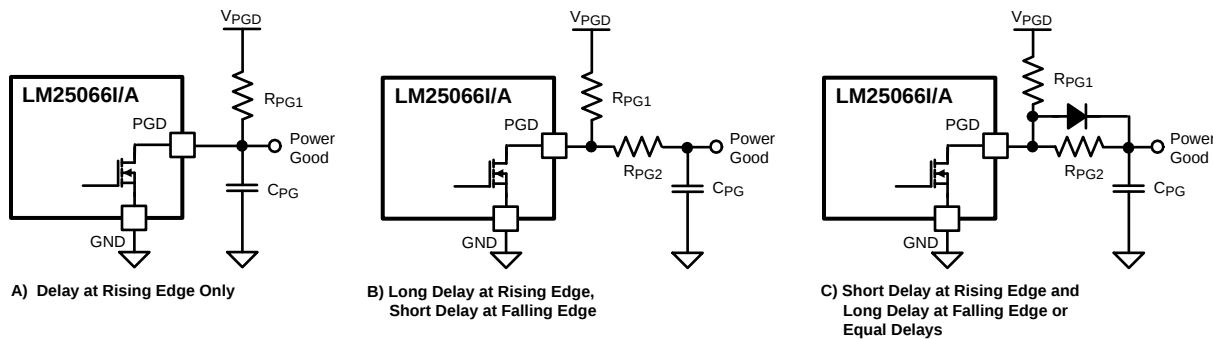
Figure 46. Adding Delay to the Power Good Output Pin
