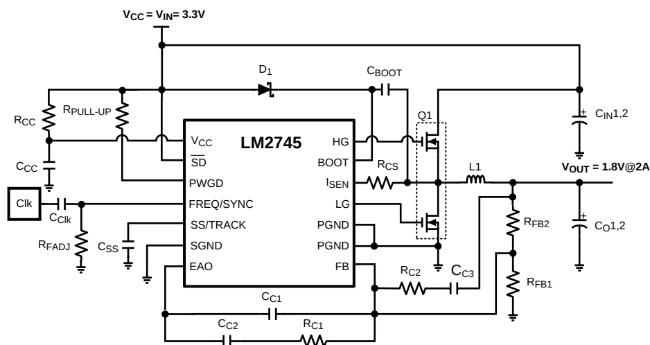
Figure 33. 3.3V to 1.8V @ 2A, f_{SW} = 300 \text{ kHz}
