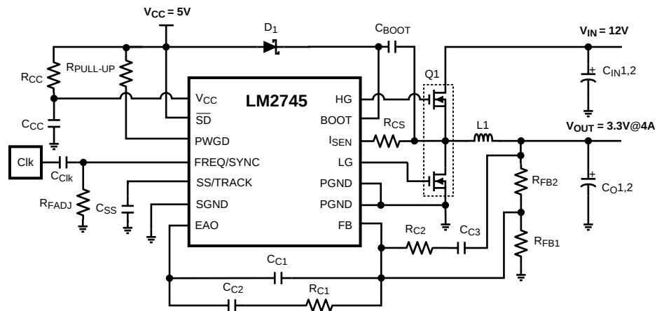
Figure 35. 12V to 3.3V @ 4A, f_{SW} = 300\text{kHz}
