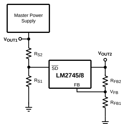
Figure 22. Sequencing Circuit
