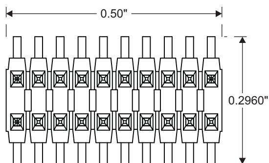
Figure 3. TI 20-Pin CTI Header
