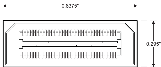
Figure 2. MIPI 60-Pin Header
