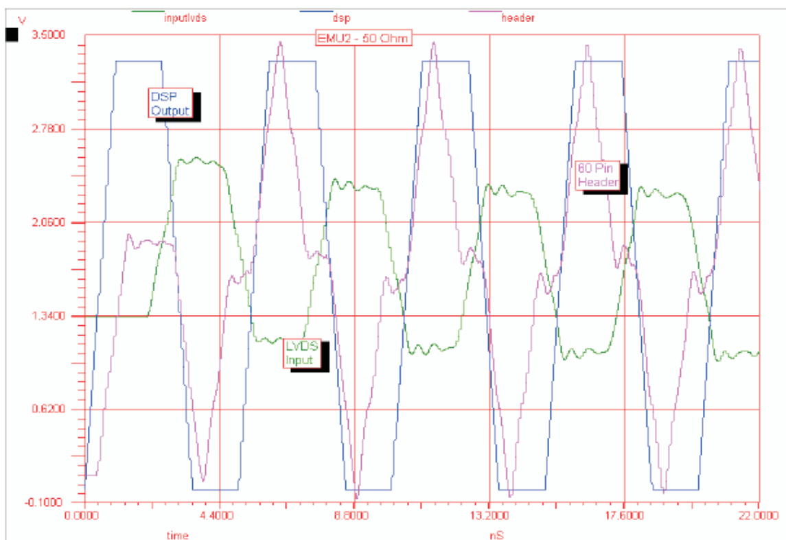
Figure 37. EMU2 Type Signals Acceptable Wave Form (Host Side, TI's XDS560T Pod - 50 \Omega )
