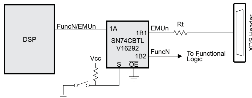
Figure 22. Multi-Function Trace
