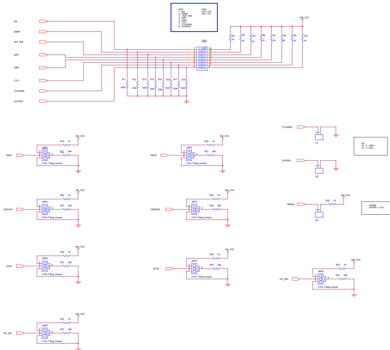
Figure 5. TUSB544RNQEVMSchematic (Page 2)
