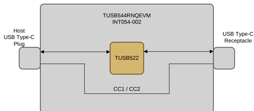
Figure 3. TUSB544RNQEVMSchematic Block Diagram
