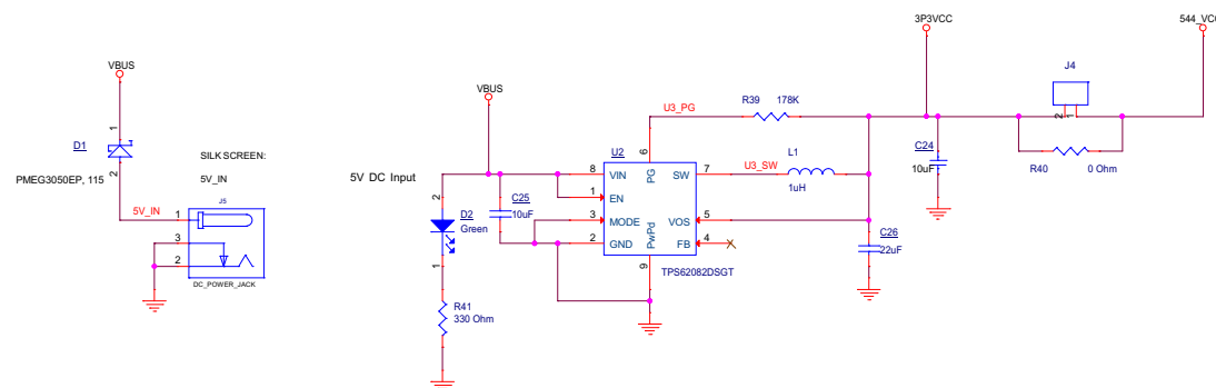
Figure 6. TUSB544RNQEVM Schematic (Page 3)
