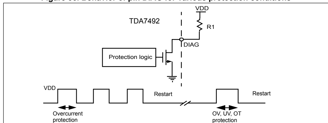
Figure 35. Behavior of pin DIAG for various protection conditions
