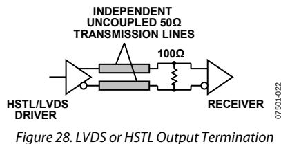
Figure 28. LVDS or HSTL Output Termination
