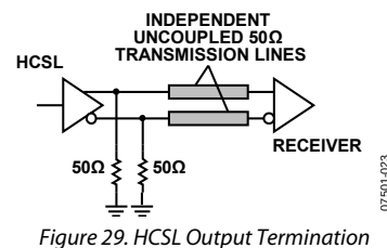
Figure 29. HCSL Output Termination
