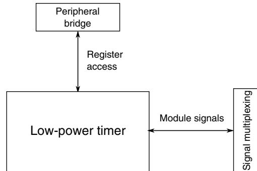
Figure 3-47. LPT configuration
