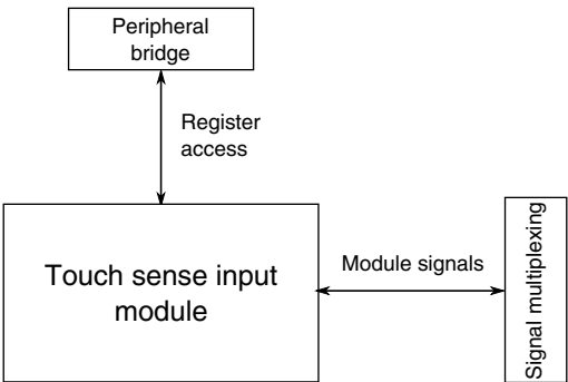
Figure 3-64. TSI configuration
