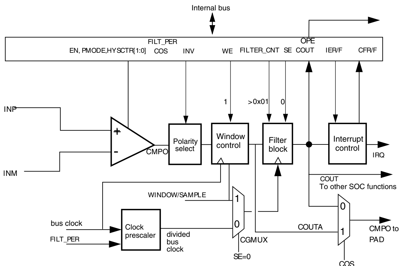
Figure 34-35. Windowed/Filtered mode
