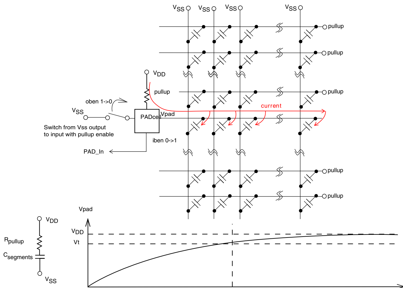
Figure 55-33. Pullup fault detect in connection/segment normal case
