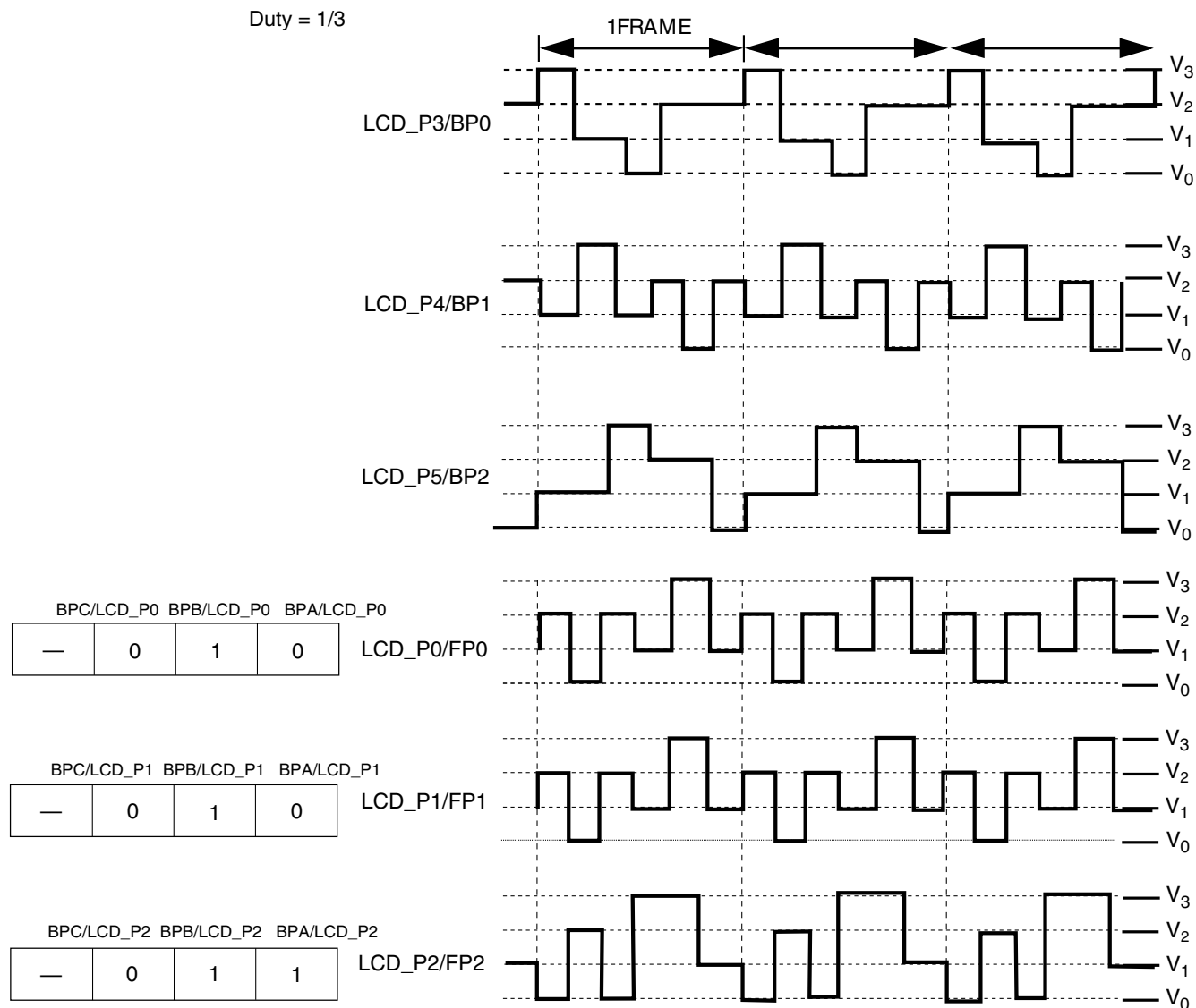
Figure 55-40. LCD waveforms
