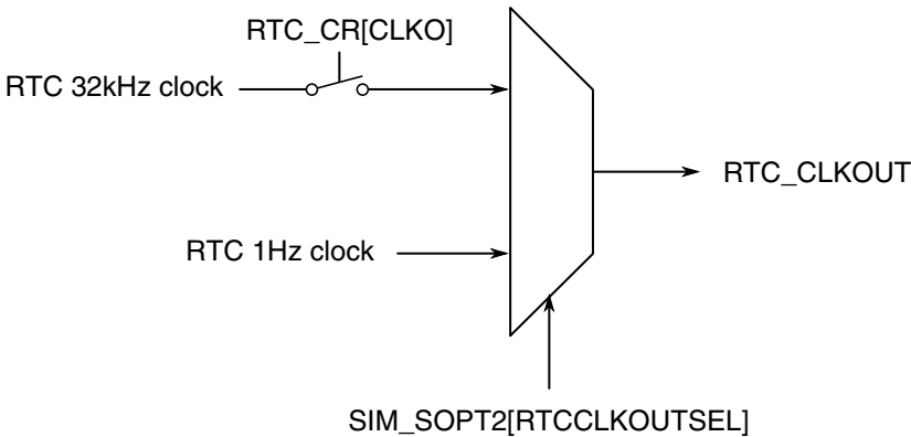
Figure 3-50. RTC_CLKOUT generation
