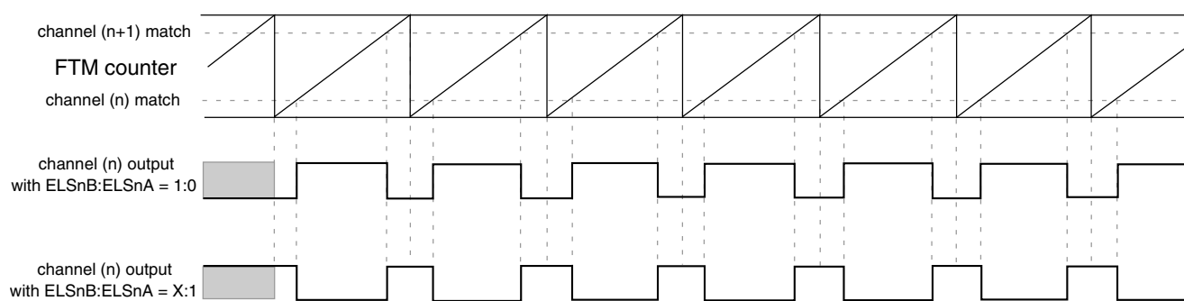
Figure 40-187. Combine mode
