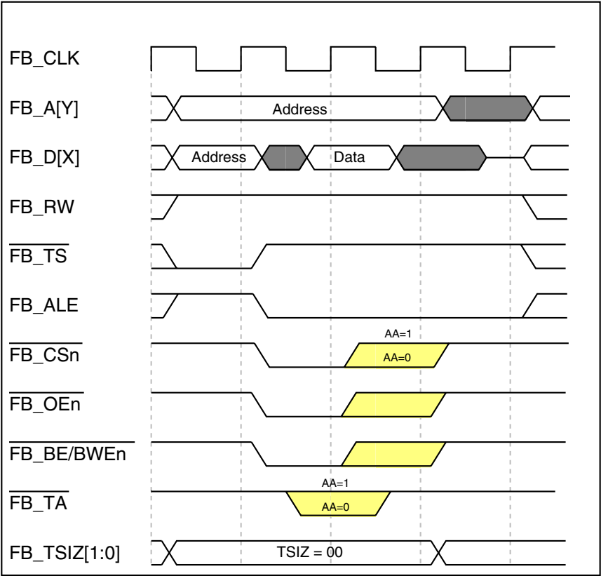
Figure 30-33. Longword-Read Transfer
