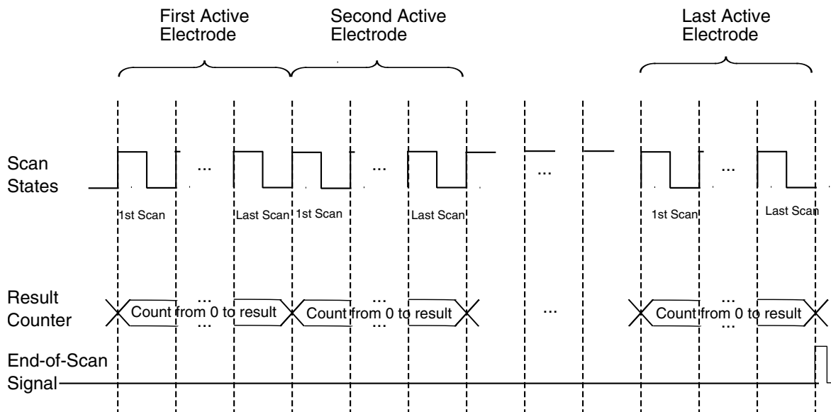
Figure 54-41. Scan sequence
