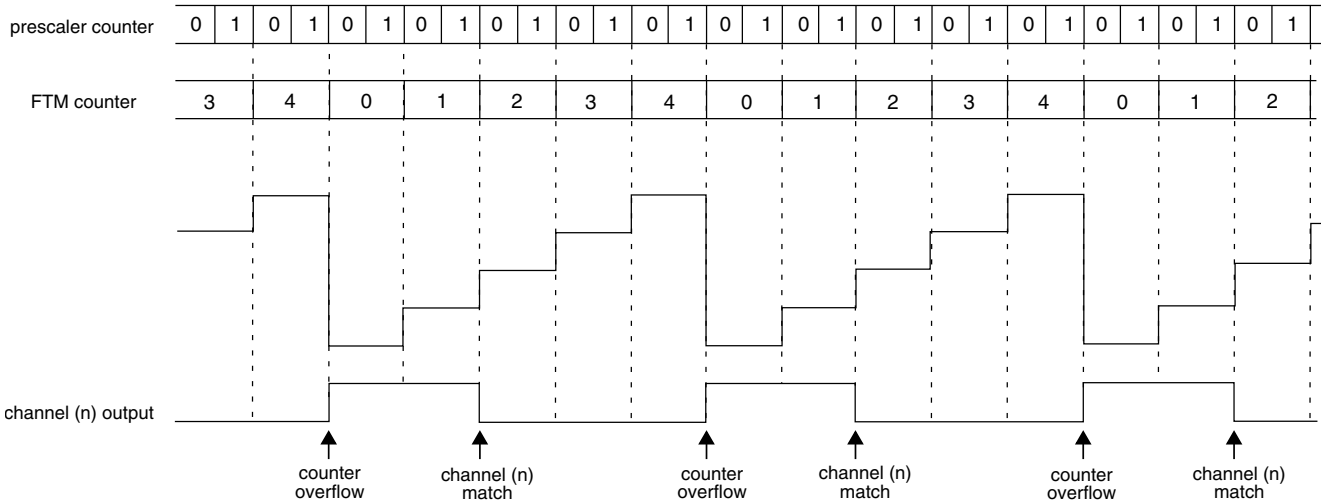
Figure 40-166. Notation used
