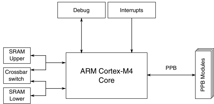
Figure 3-1. Core configuration
