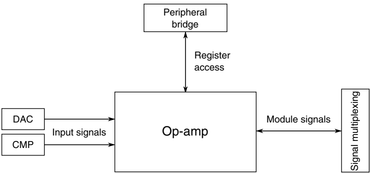
Figure 3-39. Op-amp configuration
