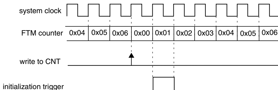
Figure 40-240. Initialization trigger is generated when there is a write to CNT register
