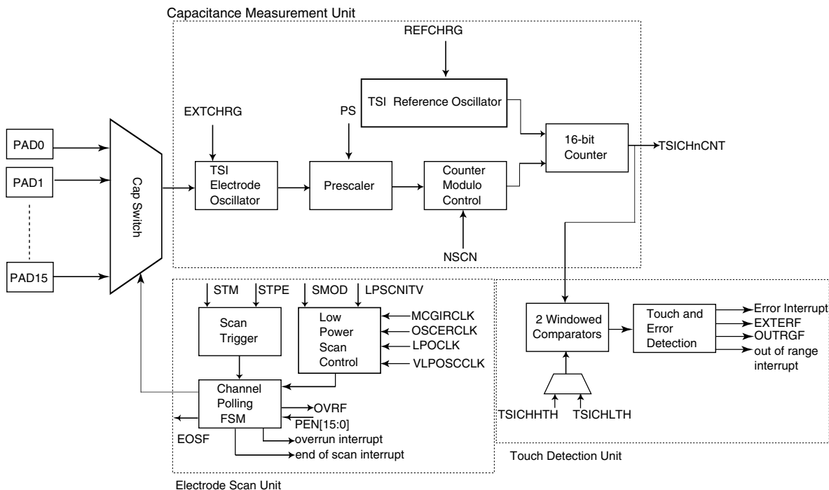
Figure 54-3. TSI block diagram
